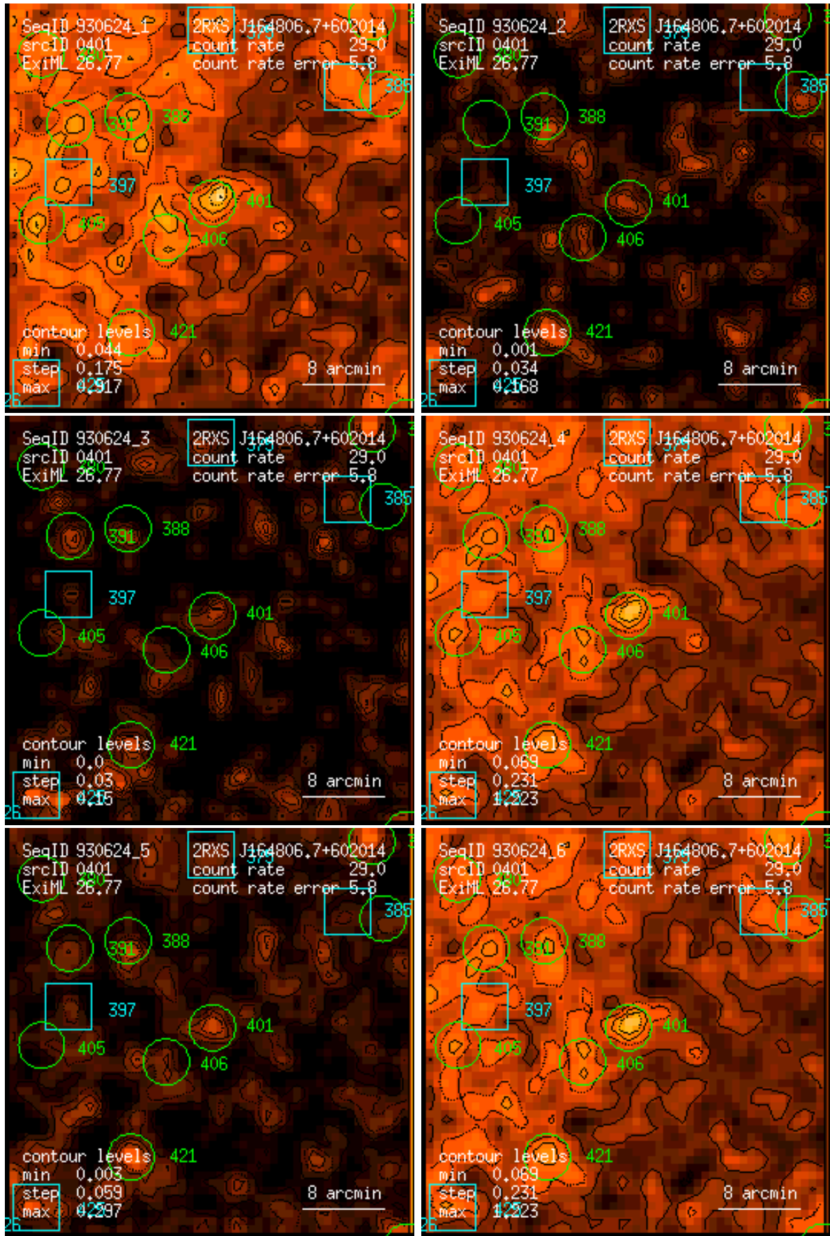
Figure 401: RASS 930624: detection 0401: band rate images, Gaussian filter: (1) PSPC channels 11 – 41, (2) 52 – 90, (3) 91 – 201, (4) 11 – 235, (5) 52 – 201, (6) 11 – 201. Broad band rates in counts/ks. Band rate contour levels in counts/ks/arcmin 2 .
