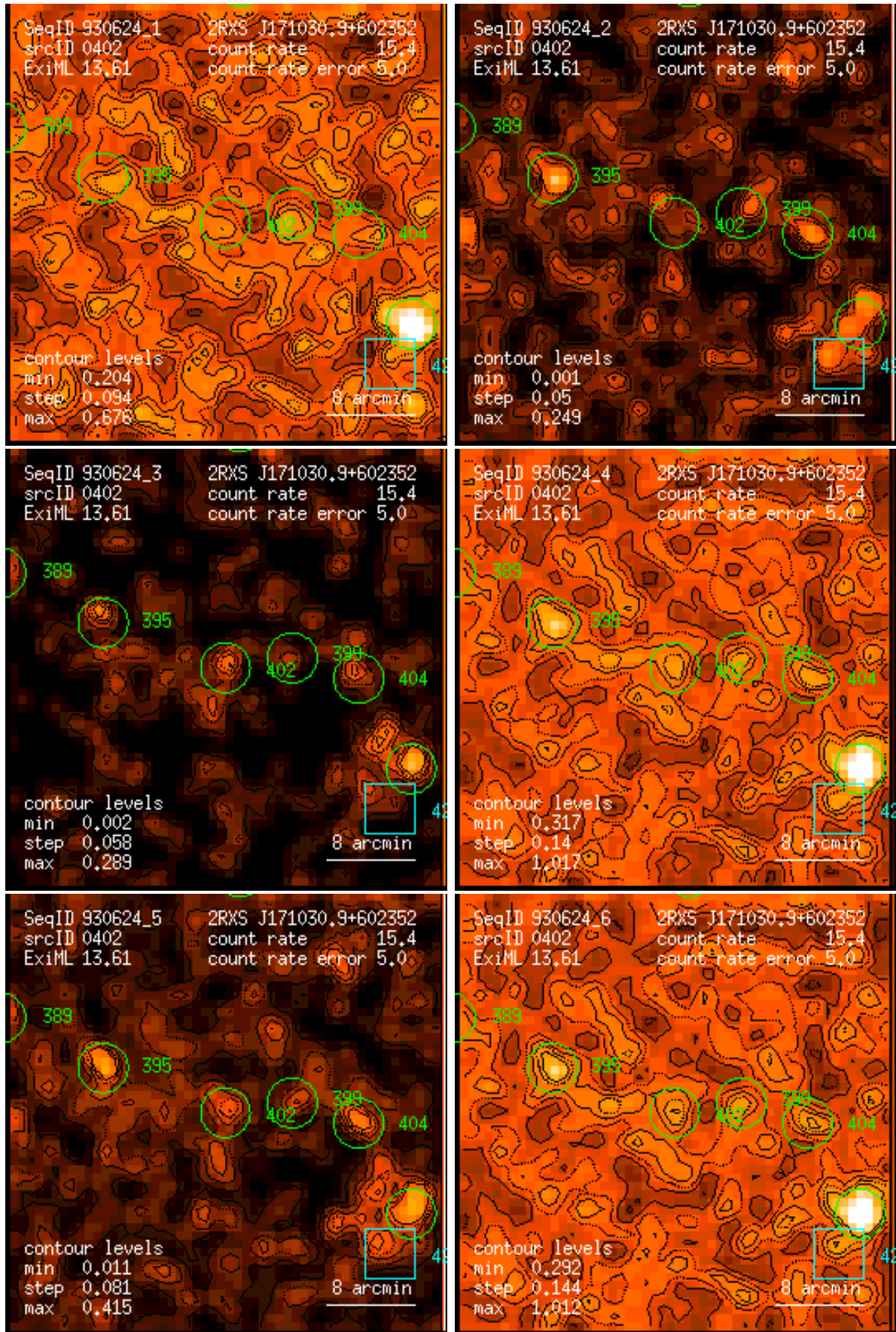
Figure 402: RASS 930624: detection 0402: band rate images, Gaussian filter: (1) PSPC channels 11 – 41, (2) 52 – 90, (3) 91 – 201, (4) 11 – 235, (5) 52 – 201, (6) 11 – 201. Broad band rates in counts/ks. Band rate contour levels in counts/ks/arcmin 2 .
