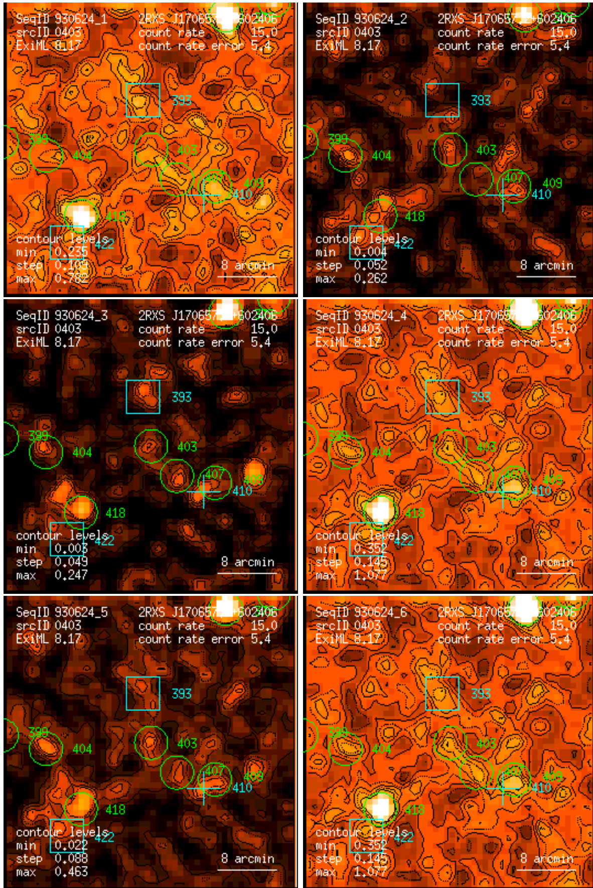
Figure 403: RASS 930624: detection 0403: band rate images, Gaussian filter: (1) PSPC channels 11 – 41, (2) 52 – 90, (3) 91 – 201, (4) 11 – 235, (5) 52 – 201, (6) 11 – 201. Broad band rates in counts/ks. Band rate contour levels in counts/ks/arcmin 2 .
