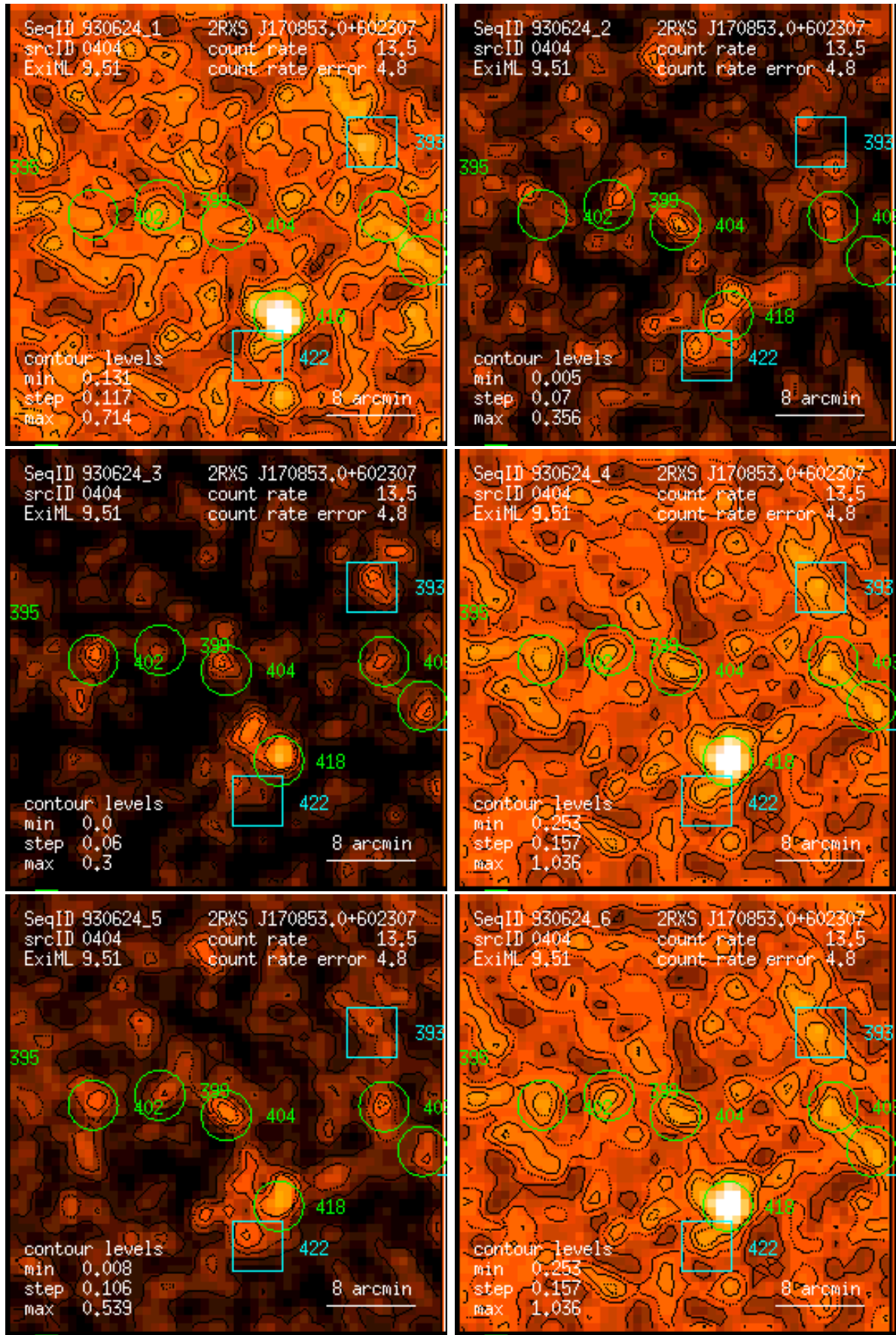
Figure 404: RASS 930624: detection 0404: band rate images, Gaussian filter: (1) PSPC channels 11 – 41, (2) 52 – 90, (3) 91 – 201, (4) 11 – 235, (5) 52 – 201, (6) 11 – 201. Broad band rates in counts/ks. Band rate contour levels in counts/ks/arcmin 2 .
