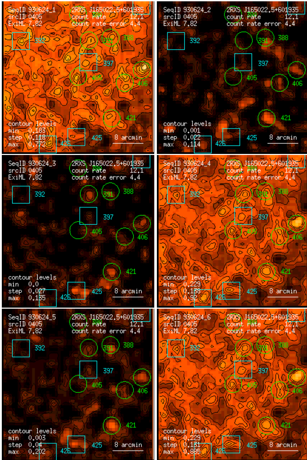
Figure 405: RASS 930624: detection 0405: band rate images, Gaussian filter: (1) PSPC channels 11 – 41, (2) 52 – 90, (3) 91 – 201, (4) 11 – 235, (5) 52 – 201, (6) 11 – 201. Broad band rates in counts/ks. Band rate contour levels in counts/ks/arcmin 2 .
