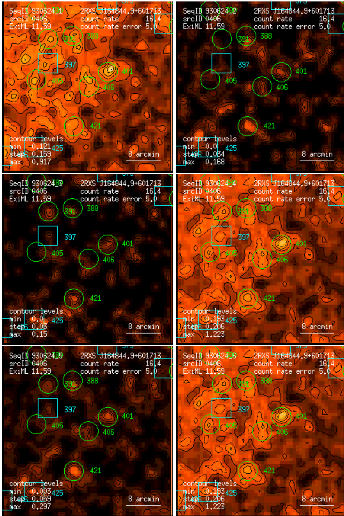
Figure 406: RASS 930624: detection 0406: band rate images, Gaussian filter: (1) PSPC channels 11 – 41, (2) 52 – 90, (3) 91 – 201, (4) 11 – 235, (5) 52 – 201, (6) 11 – 201. Broad band rates in counts/ks. Band rate contour levels in counts/ks/arcmin 2 .
