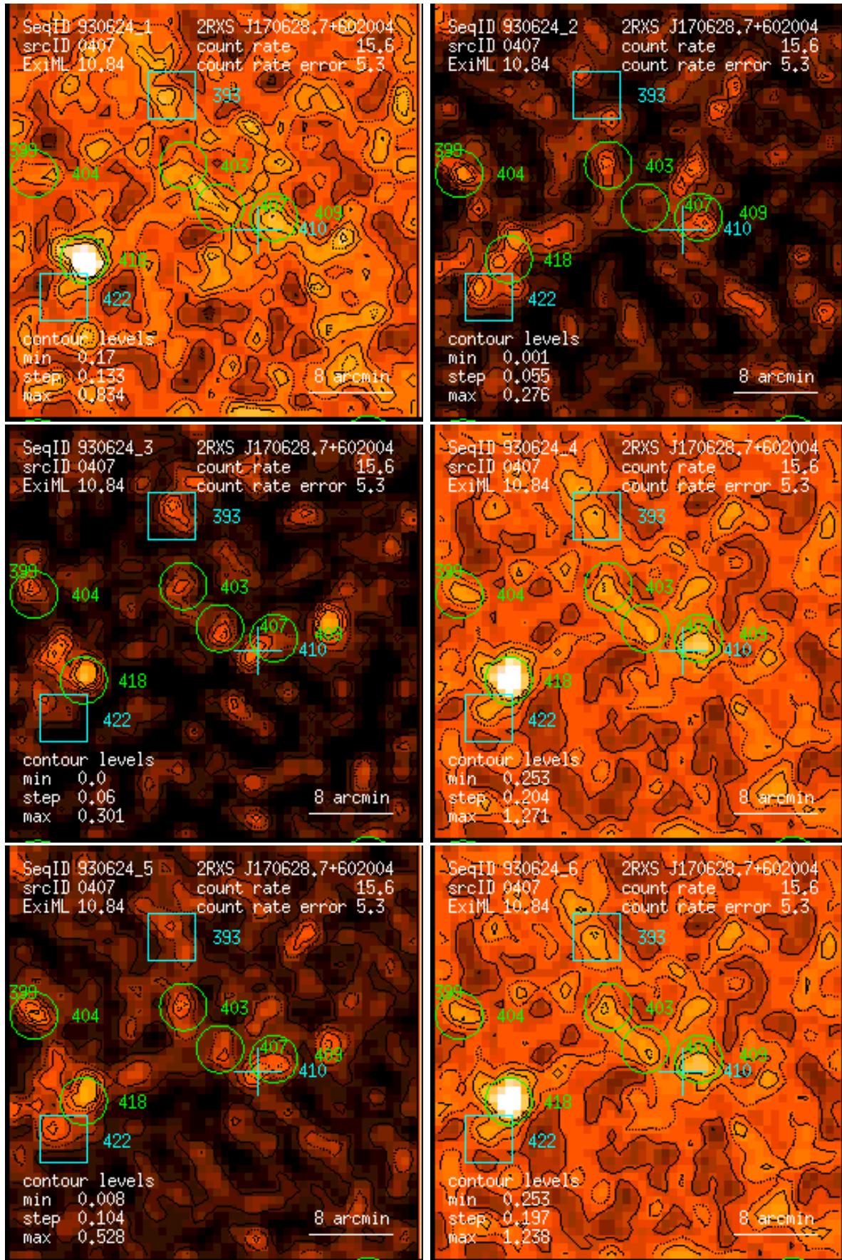
Figure 407: RASS 930624: detection 0407: band rate images, Gaussian filter: (1) PSPC channels 11 – 41, (2) 52 – 90, (3) 91 – 201, (4) 11 – 235, (5) 52 – 201, (6) 11 – 201. Broad band rates in counts/ks. Band rate contour levels in counts/ks/arcmin 2 .
