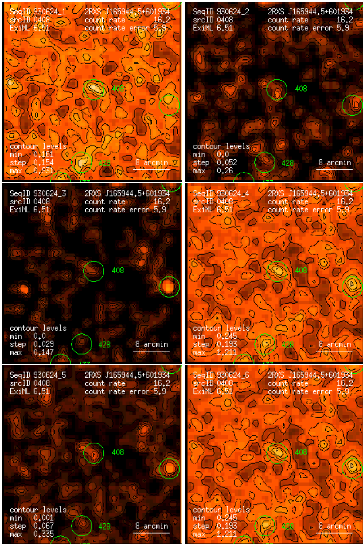
Figure 408: RASS 930624: detection 0408: band rate images, Gaussian filter: (1) PSPC channels 11 – 41, (2) 52 – 90, (3) 91 – 201, (4) 11 – 235, (5) 52 – 201, (6) 11 – 201. Broad band rates in counts/ks. Band rate contour levels in counts/ks/arcmin 2 .
