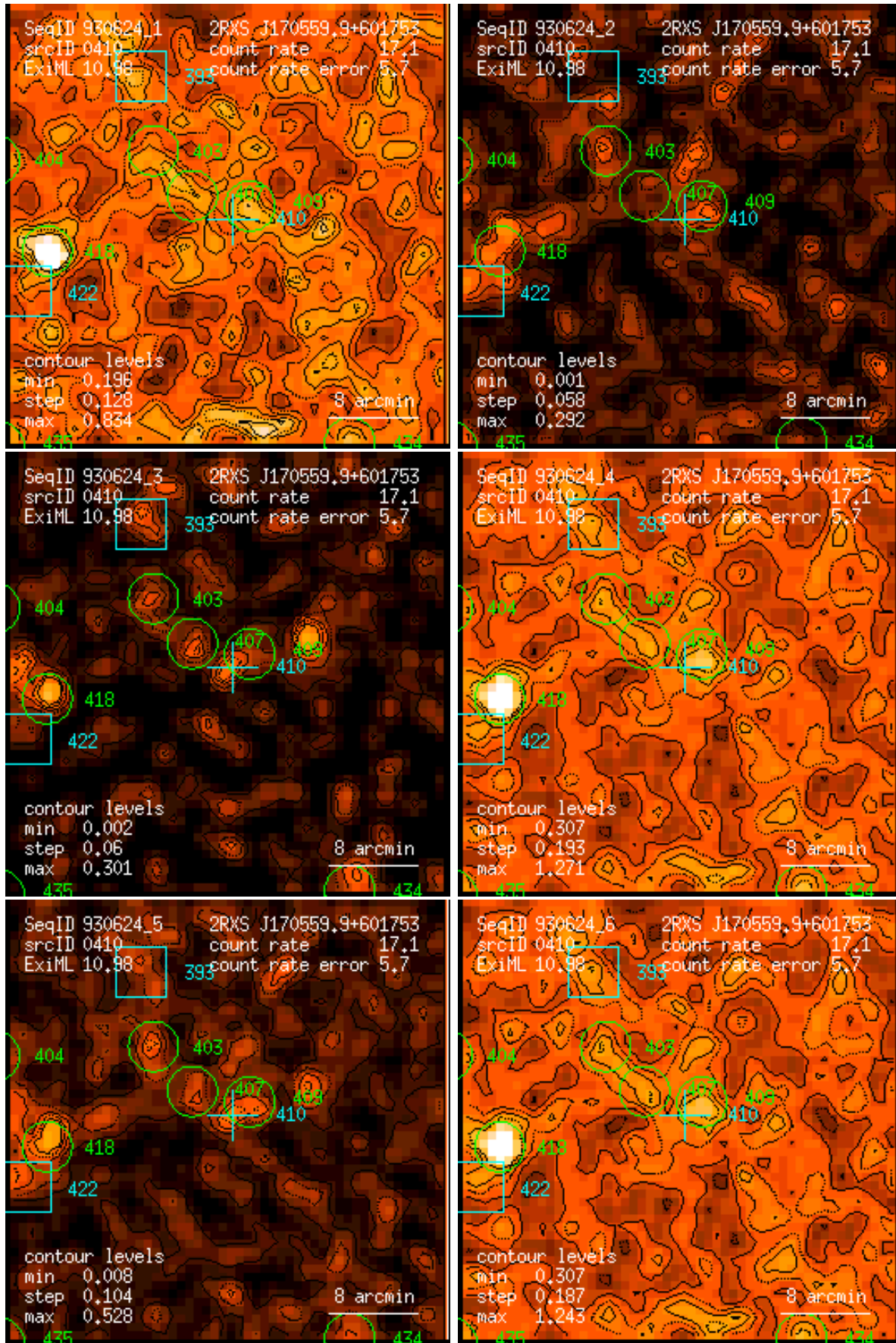
Figure 410: RASS 930624: detection 0410: band rate images, Gaussian filter: (1) PSPC channels 11 – 41, (2) 52 – 90, (3) 91 – 201, (4) 11 – 235, (5) 52 – 201, (6) 11 – 201. Broad band rates in counts/ks. Band rate contour levels in counts/ks/arcmin 2 .
