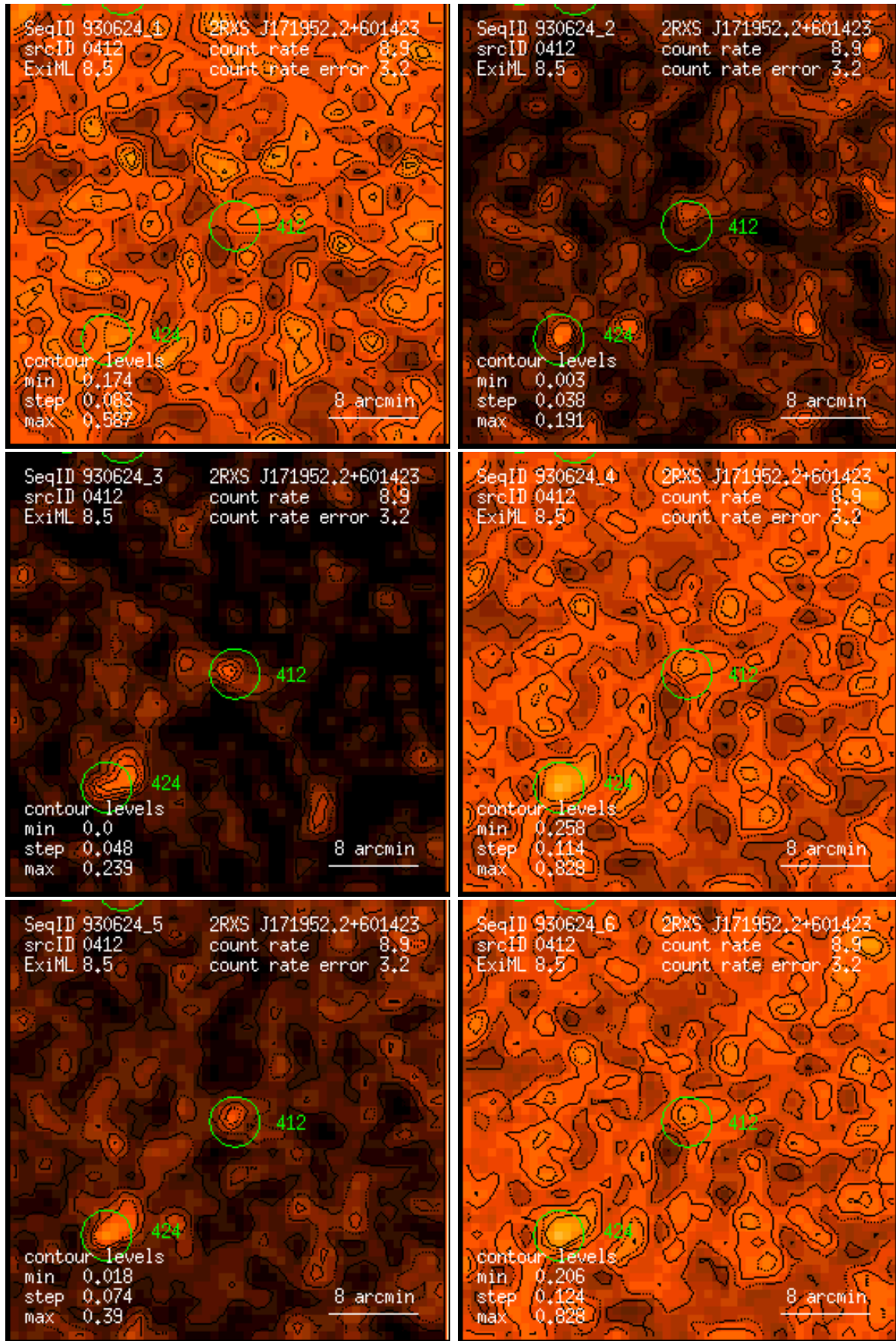
Figure 412: RASS 930624: detection 0412: band rate images, Gaussian filter: (1) PSPC channels 11 – 41, (2) 52 – 90, (3) 91 – 201, (4) 11 – 235, (5) 52 – 201, (6) 11 – 201. Broad band rates in counts/ks. Band rate contour levels in counts/ks/arcmin 2 .
