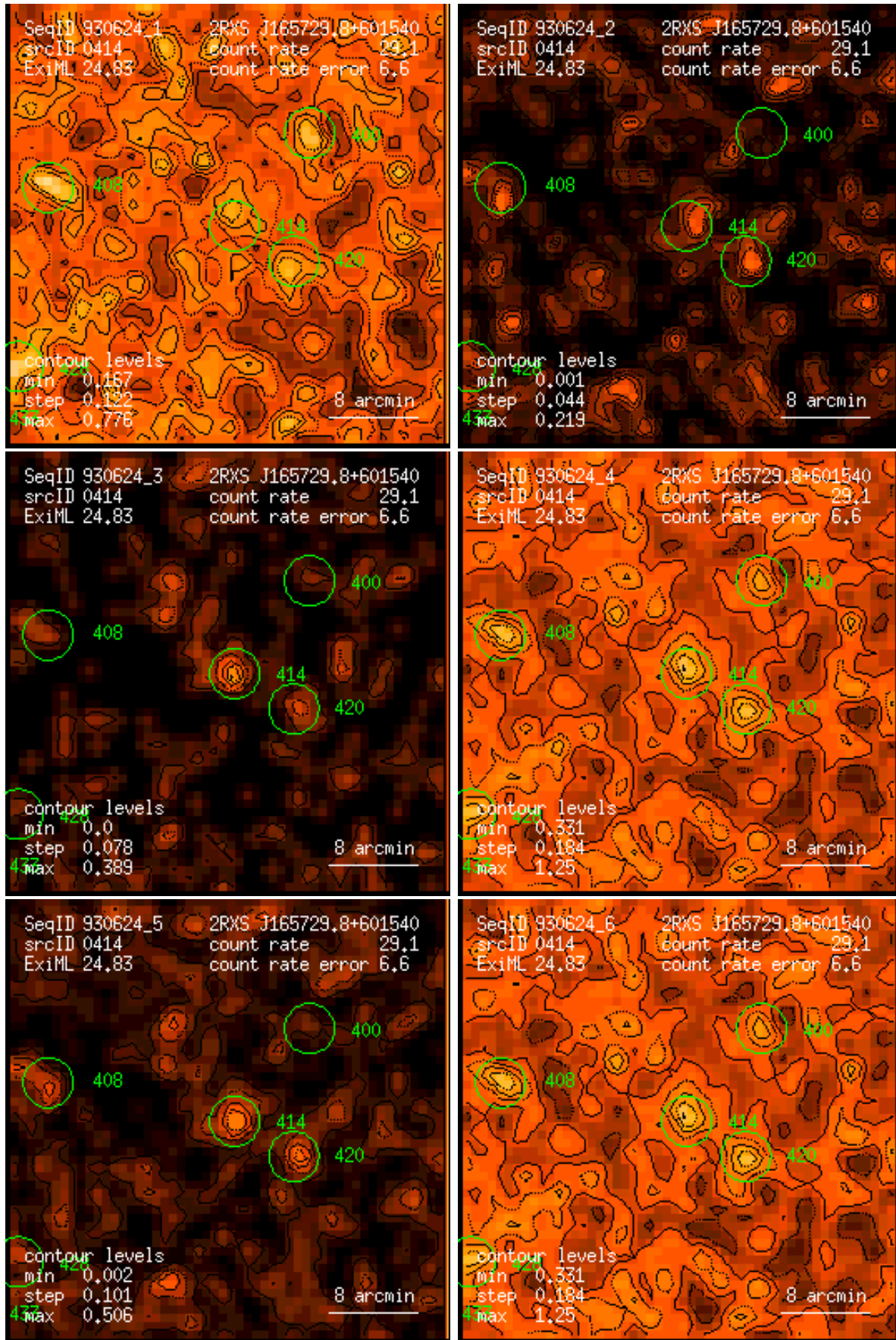
Figure 414: RASS 930624: detection 0414: band rate images, Gaussian filter: (1) PSPC channels 11 – 41, (2) 52 – 90, (3) 91 – 201, (4) 11 – 235, (5) 52 – 201, (6) 11 – 201. Broad band rates in counts/ks. Band rate contour levels in counts/ks/arcmin 2 .
