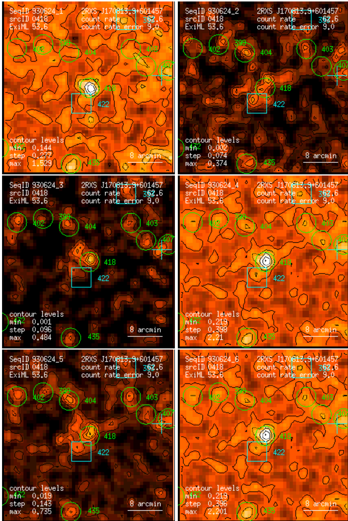
Figure 418: RASS 930624: detection 0418: band rate images, Gaussian filter: (1) PSPC channels 11 – 41, (2) 52 – 90, (3) 91 – 201, (4) 11 – 235, (5) 52 – 201, (6) 11 – 201. Broad band rates in counts/ks. Band rate contour levels in counts/ks/arcmin 2 .
