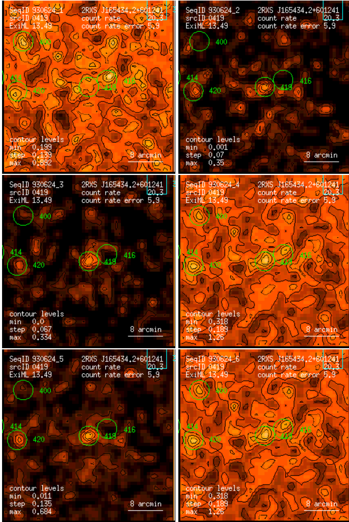
Figure 419: RASS 930624: detection 0419: band rate images, Gaussian filter: (1) PSPC channels 11 – 41, (2) 52 – 90, (3) 91 – 201, (4) 11 – 235, (5) 52 – 201, (6) 11 – 201. Broad band rates in counts/ks. Band rate contour levels in counts/ks/arcmin 2 .
