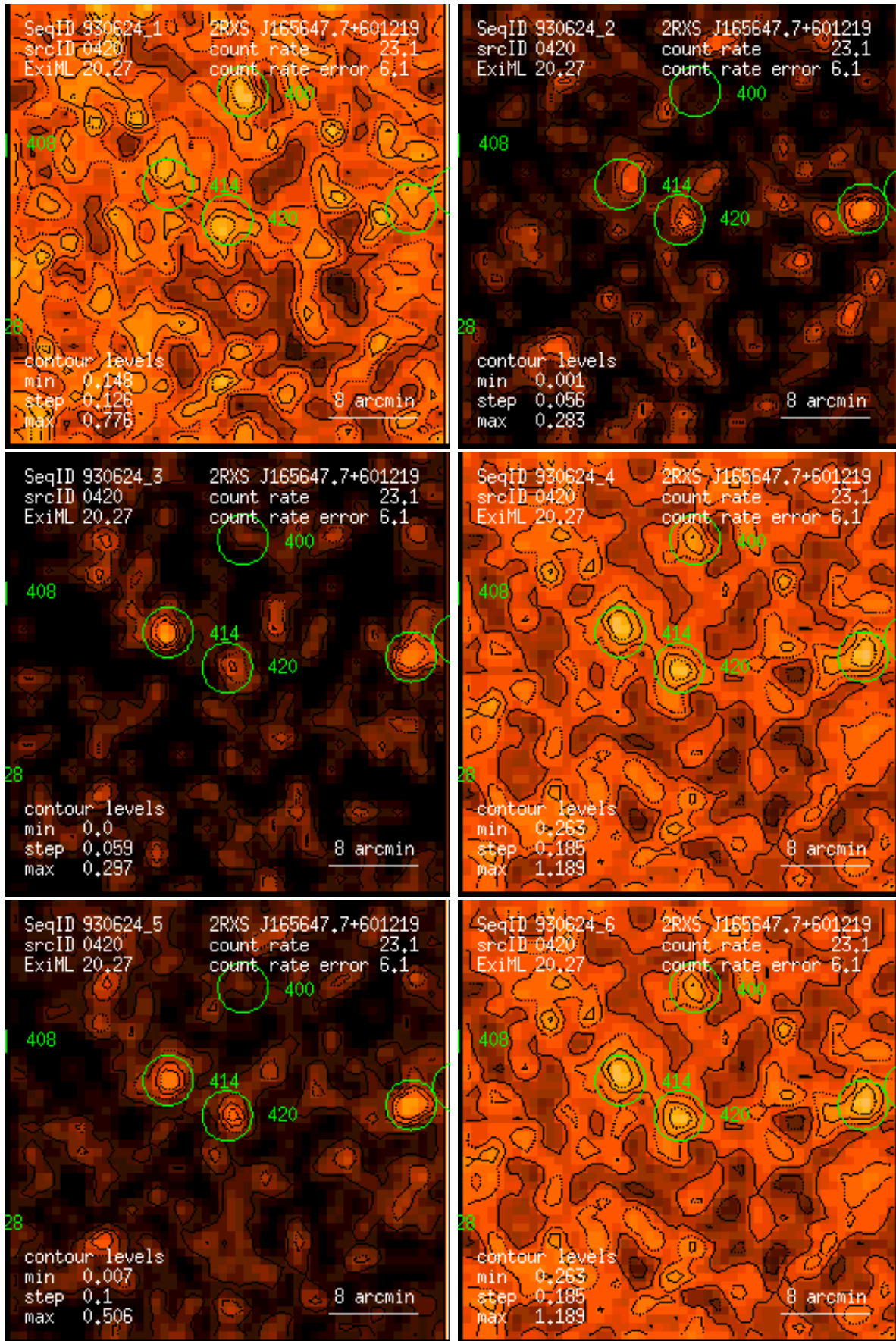
Figure 420: RASS 930624: detection 0420: band rate images, Gaussian filter: (1) PSPC channels 11 – 41, (2) 52 – 90, (3) 91 – 201, (4) 11 – 235, (5) 52 – 201, (6) 11 – 201. Broad band rates in counts/ks. Band rate contour levels in counts/ks/arcmin 2 .
