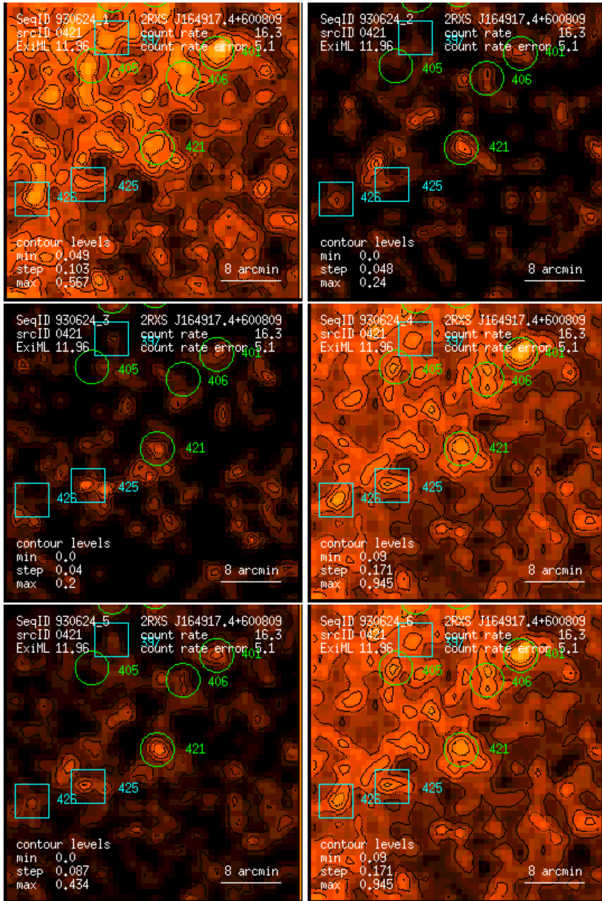
Figure 421: RASS 930624: detection 0421: band rate images, Gaussian filter: (1) PSPC channels 11 – 41, (2) 52 – 90, (3) 91 – 201, (4) 11 – 235, (5) 52 – 201, (6) 11 – 201. Broad band rates in counts/ks. Band rate contour levels in counts/ks/arcmin 2 .
