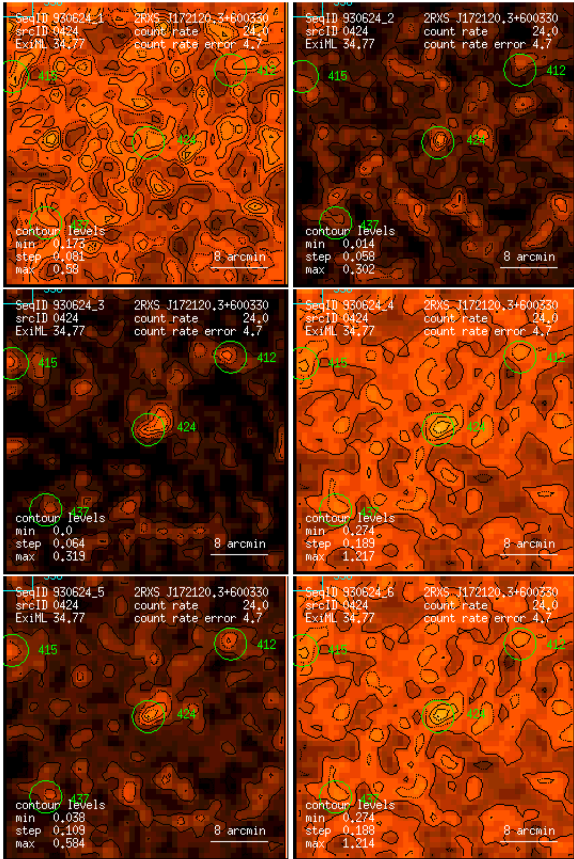
Figure 424: RASS 930624: detection 0424: band rate images, Gaussian filter: (1) PSPC channels 11 – 41, (2) 52 – 90, (3) 91 – 201, (4) 11 – 235, (5) 52 – 201, (6) 11 – 201. Broad band rates in counts/ks. Band rate contour levels in counts/ks/arcmin 2 .
