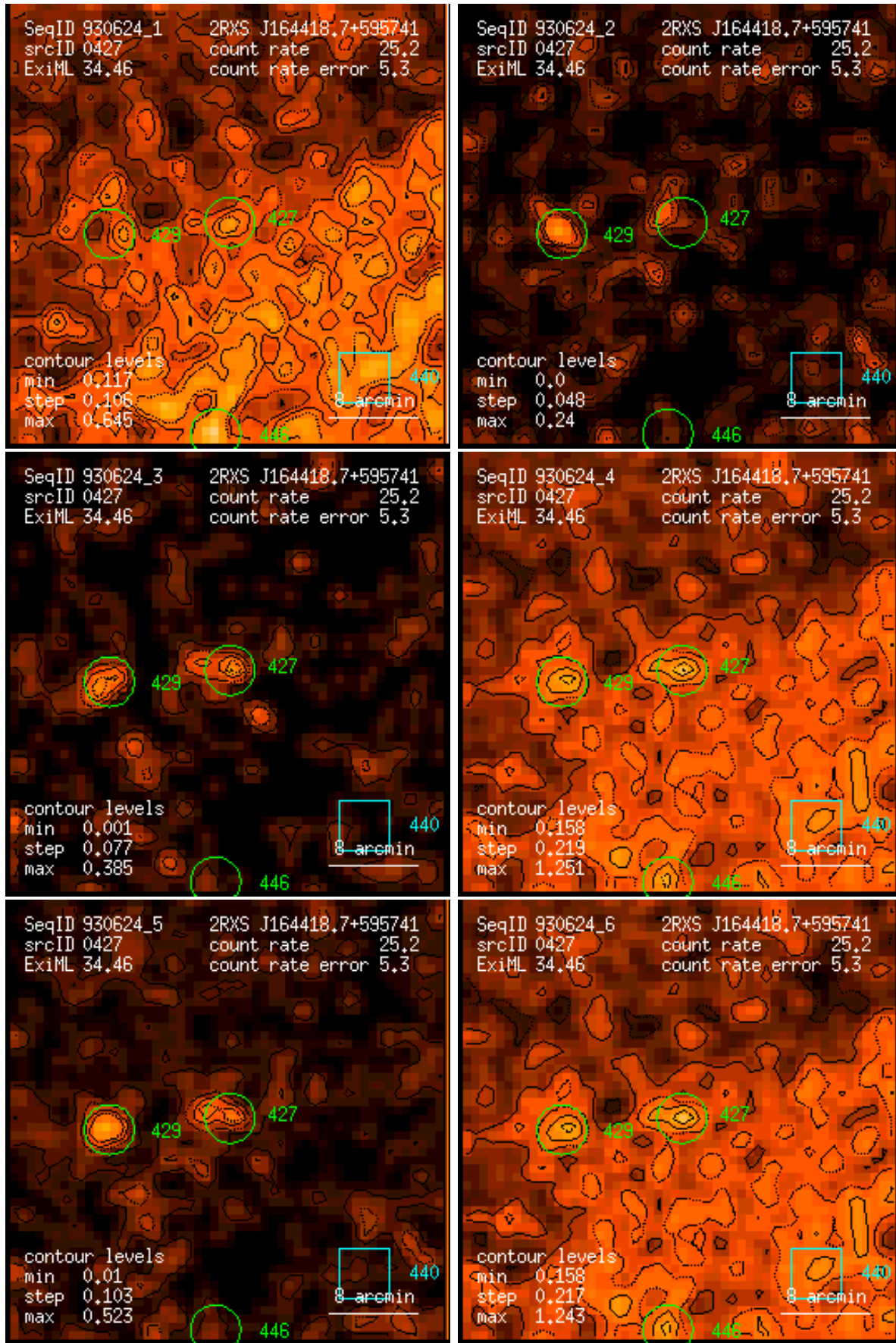
Figure 427: RASS 930624: detection 0427: band rate images, Gaussian filter: (1) PSPC channels 11 – 41, (2) 52 – 90, (3) 91 – 201, (4) 11 – 235, (5) 52 – 201, (6) 11 – 201. Broad band rates in counts/ks. Band rate contour levels in counts/ks/arcmin 2 .
