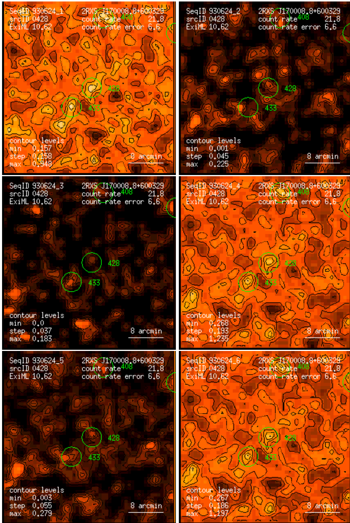
Figure 428: RASS 930624: detection 0428: band rate images, Gaussian filter: (1) PSPC channels 11 – 41, (2) 52 – 90, (3) 91 – 201, (4) 11 – 235, (5) 52 – 201, (6) 11 – 201. Broad band rates in counts/ks. Band rate contour levels in counts/ks/arcmin 2 .
