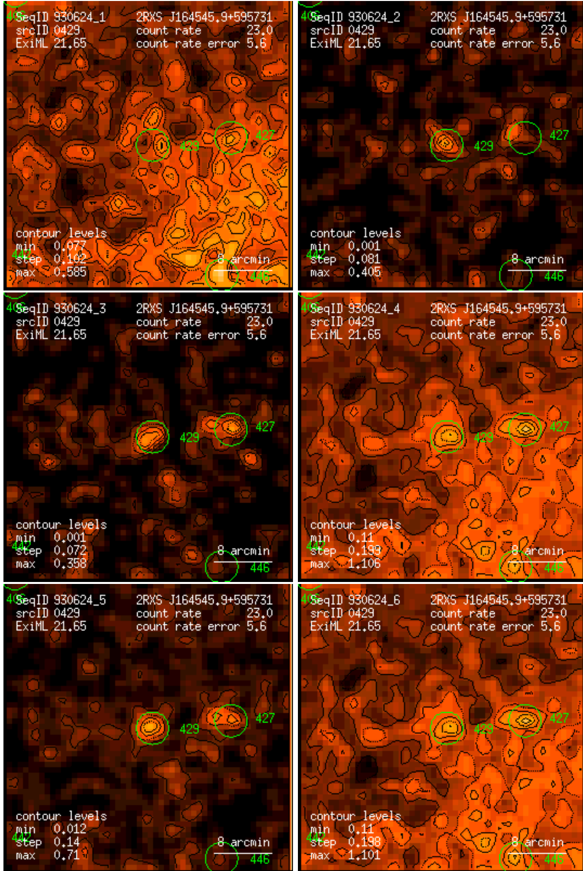
Figure 429: RASS 930624: detection 0429: band rate images, Gaussian filter: (1) PSPC channels 11 – 41, (2) 52 – 90, (3) 91 – 201, (4) 11 – 235, (5) 52 – 201, (6) 11 – 201. Broad band rates in counts/ks. Band rate contour levels in counts/ks/arcmin 2 .
