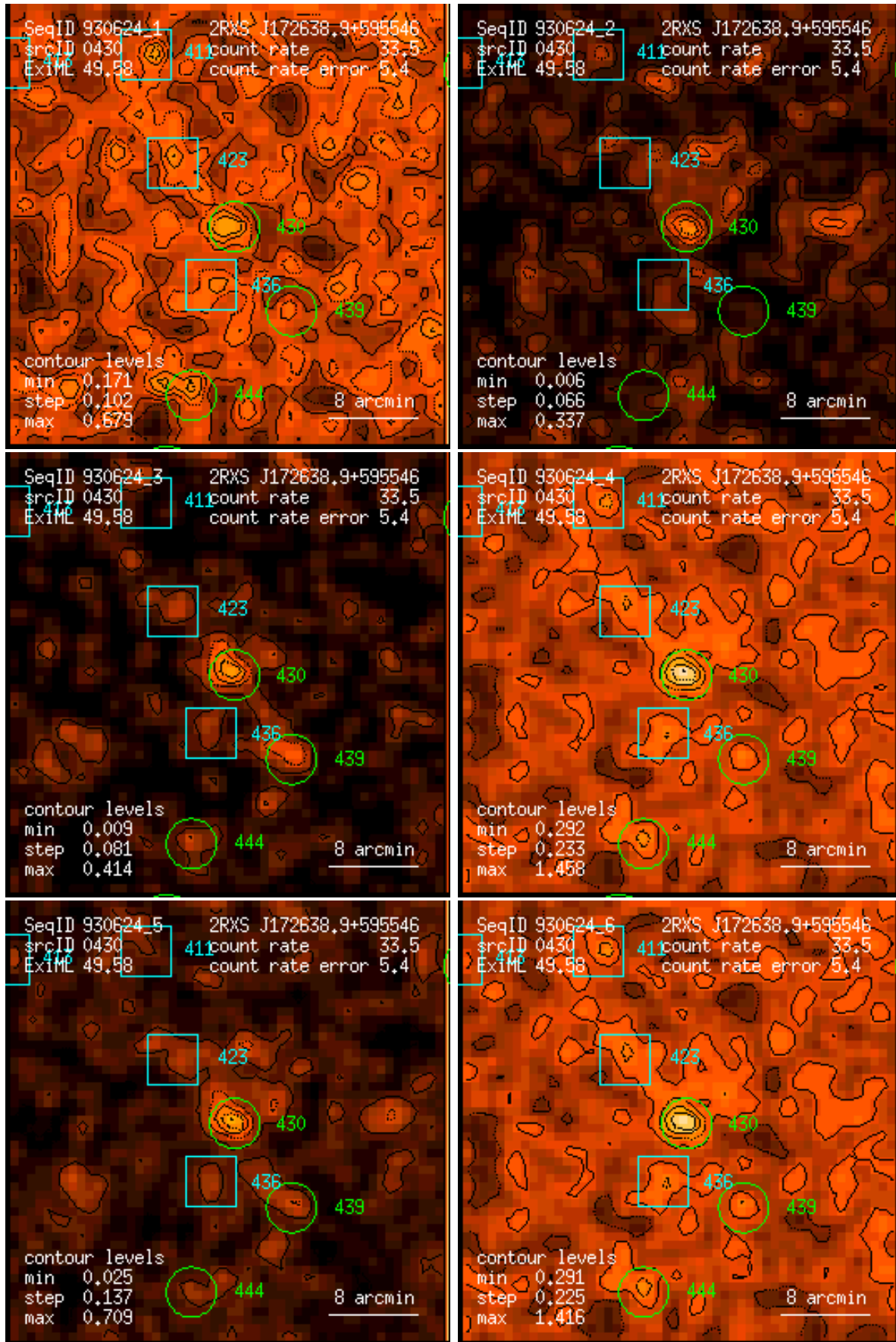
Figure 430: RASS 930624: detection 0430: band rate images, Gaussian filter: (1) PSPC channels 11 – 41, (2) 52 – 90, (3) 91 – 201, (4) 11 – 235, (5) 52 – 201, (6) 11 – 201. Broad band rates in counts/ks. Band rate contour levels in counts/ks/arcmin 2 .
