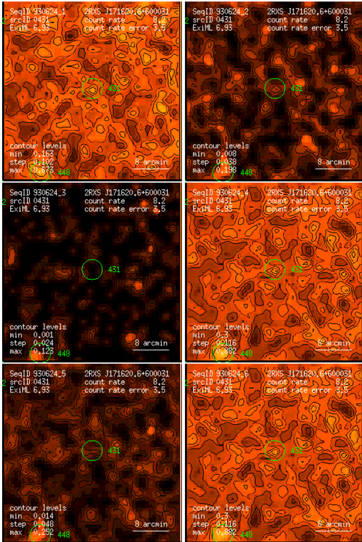
Figure 431: RASS 930624: detection 0431: band rate images, Gaussian filter: (1) PSPC channels 11 – 41, (2) 52 – 90, (3) 91 – 201, (4) 11 – 235, (5) 52 – 201, (6) 11 – 201. Broad band rates in counts/ks. Band rate contour levels in counts/ks/arcmin 2 .
