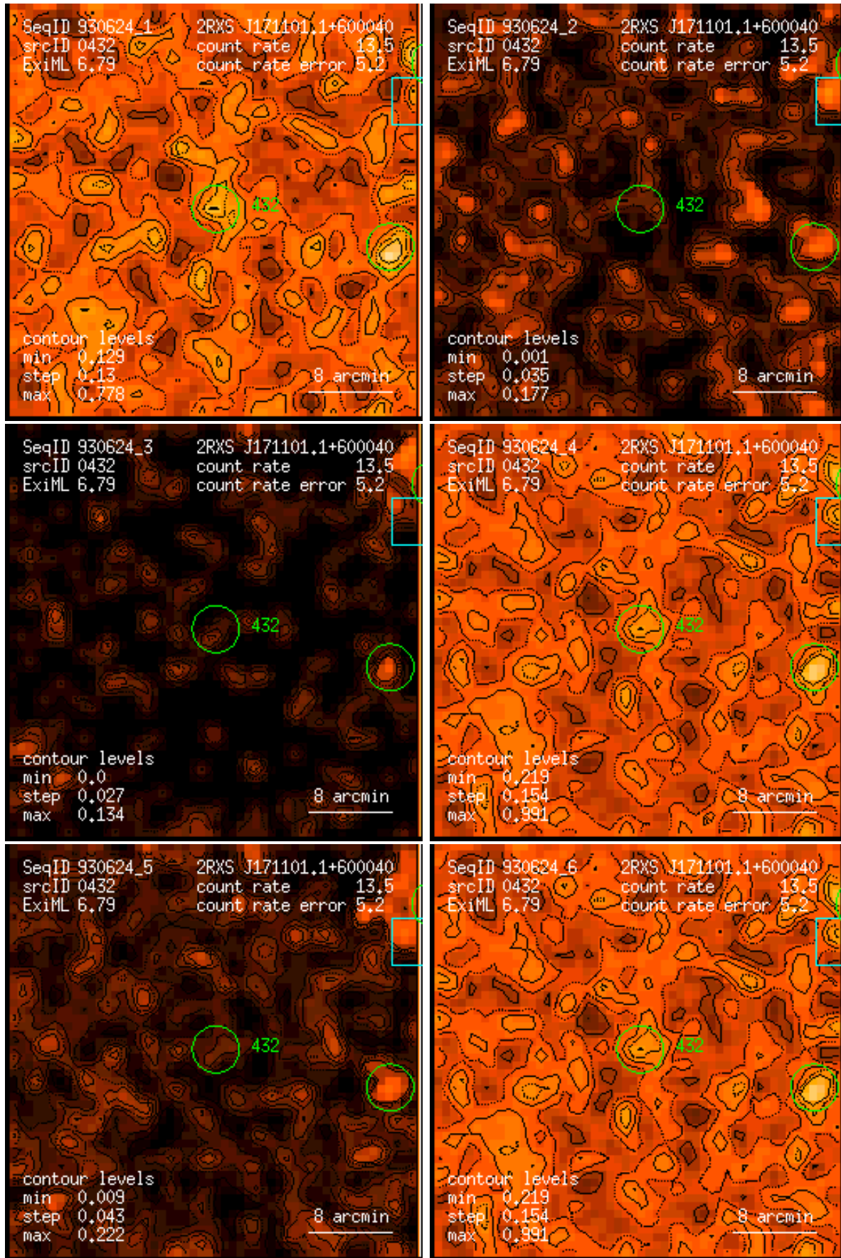
Figure 432: RASS 930624: detection 0432: band rate images, Gaussian filter: (1) PSPC channels 11 – 41, (2) 52 – 90, (3) 91 – 201, (4) 11 – 235, (5) 52 – 201, (6) 11 – 201. Broad band rates in counts/ks. Band rate contour levels in counts/ks/arcmin 2 .
