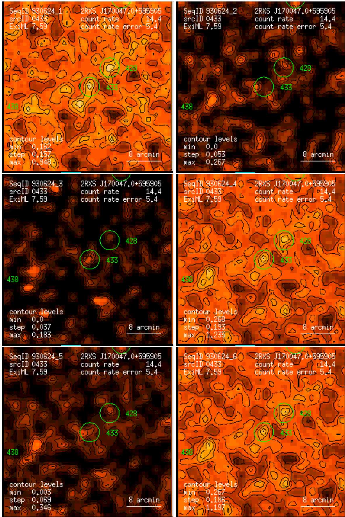
Figure 433: RASS 930624: detection 0433: band rate images, Gaussian filter: (1) PSPC channels 11 – 41, (2) 52 – 90, (3) 91 – 201, (4) 11 – 235, (5) 52 – 201, (6) 11 – 201. Broad band rates in counts/ks. Band rate contour levels in counts/ks/arcmin 2 .
