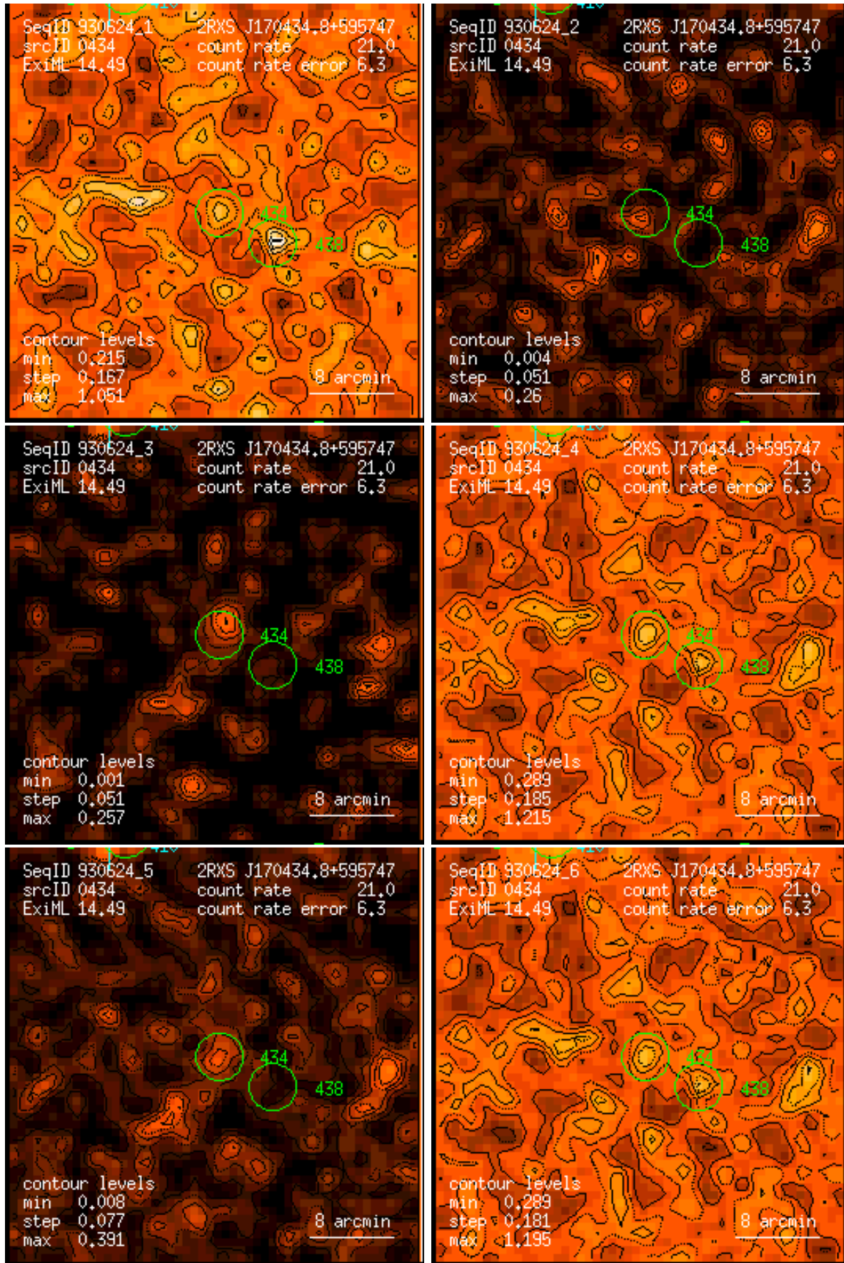
Figure 434: RASS 930624: detection 0434: band rate images, Gaussian filter: (1) PSPC channels 11 – 41, (2) 52 – 90, (3) 91 – 201, (4) 11 – 235, (5) 52 – 201, (6) 11 – 201. Broad band rates in counts/ks. Band rate contour levels in counts/ks/arcmin 2 .
