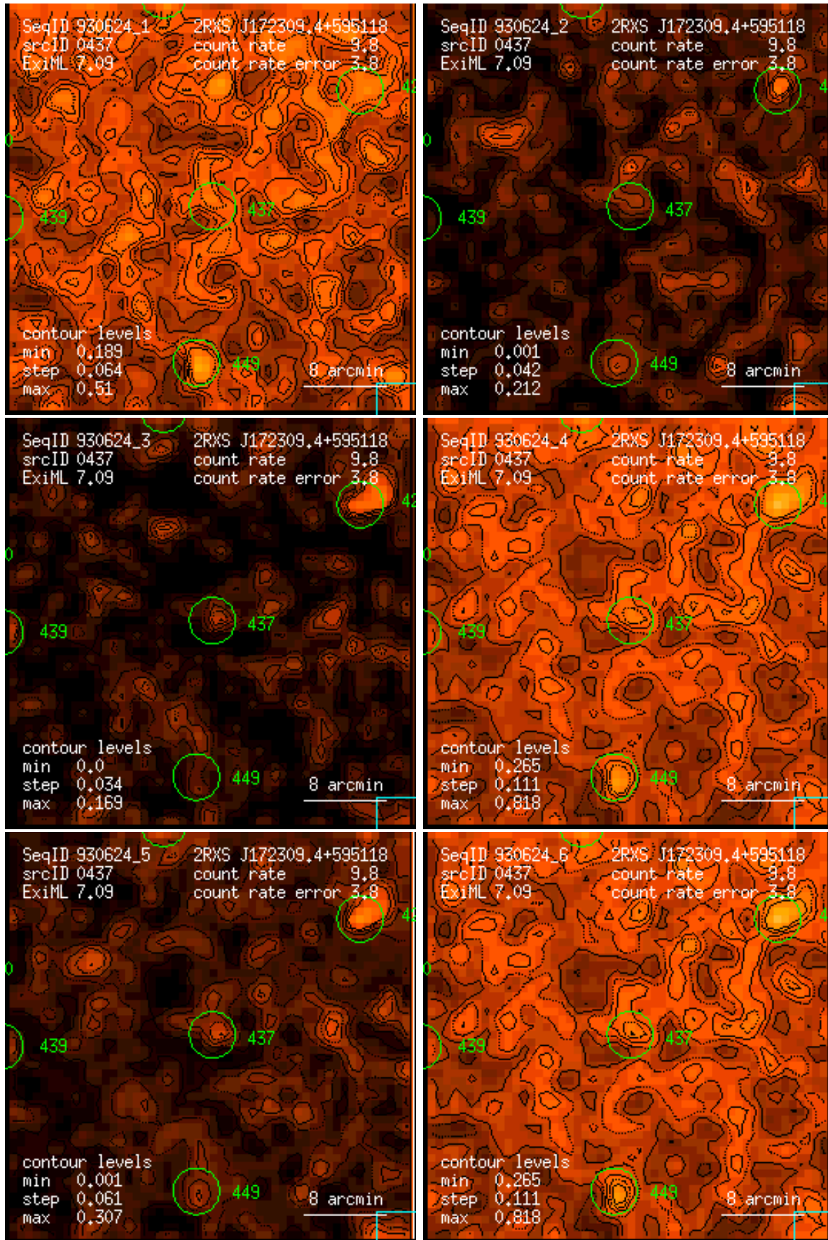
Figure 437: RASS 930624: detection 0437: band rate images, Gaussian filter: (1) PSPC channels 11 – 41, (2) 52 – 90, (3) 91 – 201, (4) 11 – 235, (5) 52 – 201, (6) 11 – 201. Broad band rates in counts/ks. Band rate contour levels in counts/ks/arcmin 2 .
