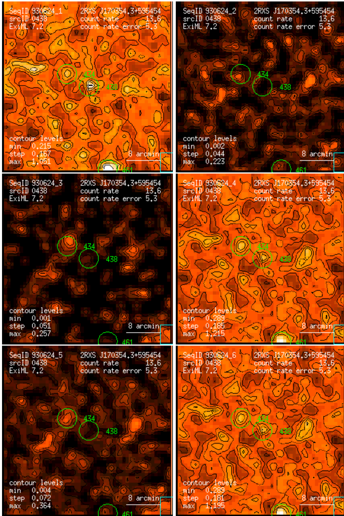
Figure 438: RASS 930624: detection 0438: band rate images, Gaussian filter: (1) PSPC channels 11 – 41, (2) 52 – 90, (3) 91 – 201, (4) 11 – 235, (5) 52 – 201, (6) 11 – 201. Broad band rates in counts/ks. Band rate contour levels in counts/ks/arcmin 2 .
