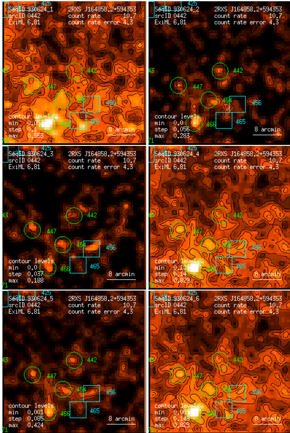
Figure 442: RASS 930624: detection 0442: band rate images, Gaussian filter: (1) PSPC channels 11 – 41, (2) 52 – 90, (3) 91 – 201, (4) 11 – 235, (5) 52 – 201, (6) 11 – 201. Broad band rates in counts/ks. Band rate contour levels in counts/ks/arcmin 2 .
