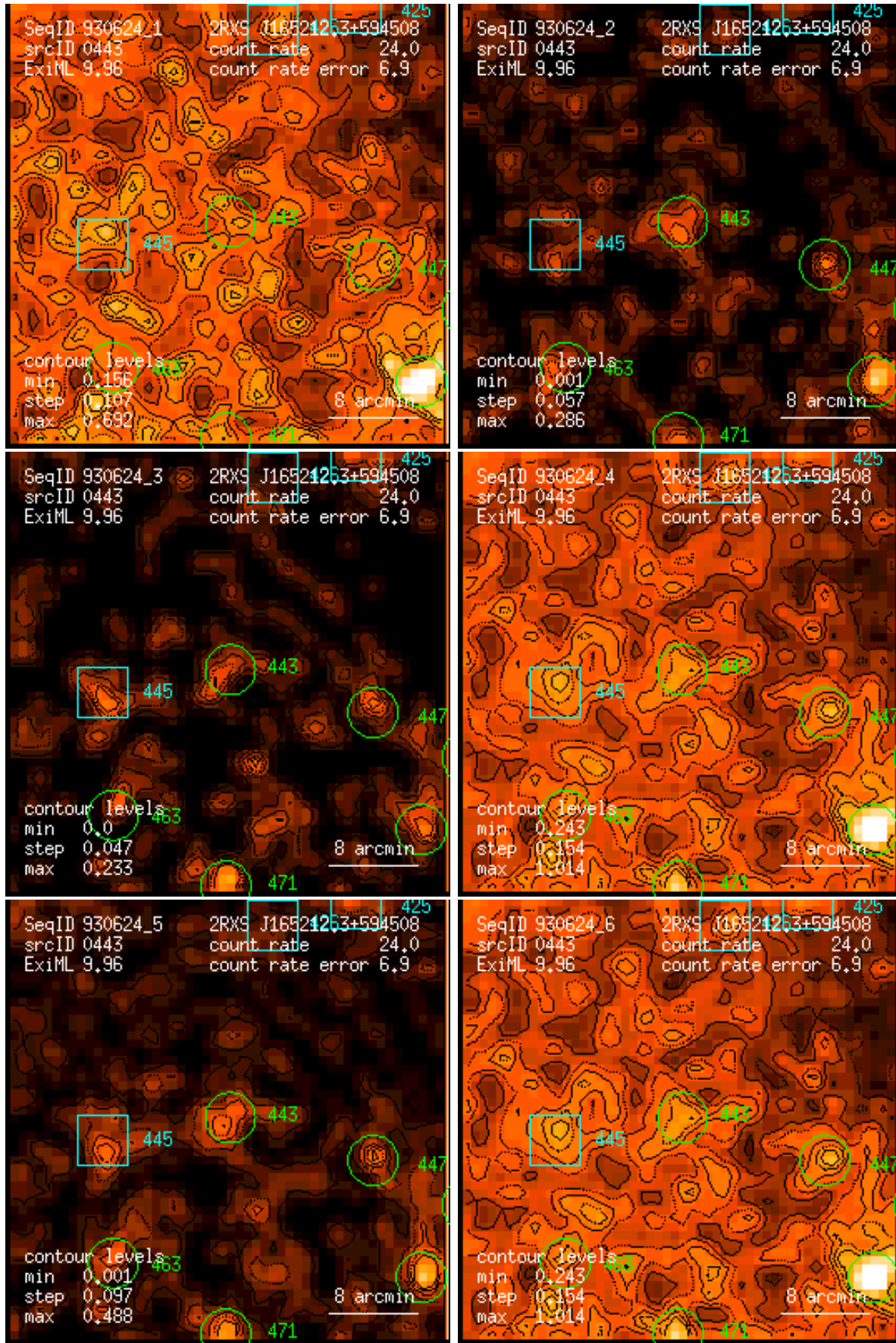
Figure 443: RASS 930624: detection 0443: band rate images, Gaussian filter: (1) PSPC channels 11 – 41, (2) 52 – 90, (3) 91 – 201, (4) 11 – 235, (5) 52 – 201, (6) 11 – 201. Broad band rates in counts/ks. Band rate contour levels in counts/ks/arcmin 2 .
