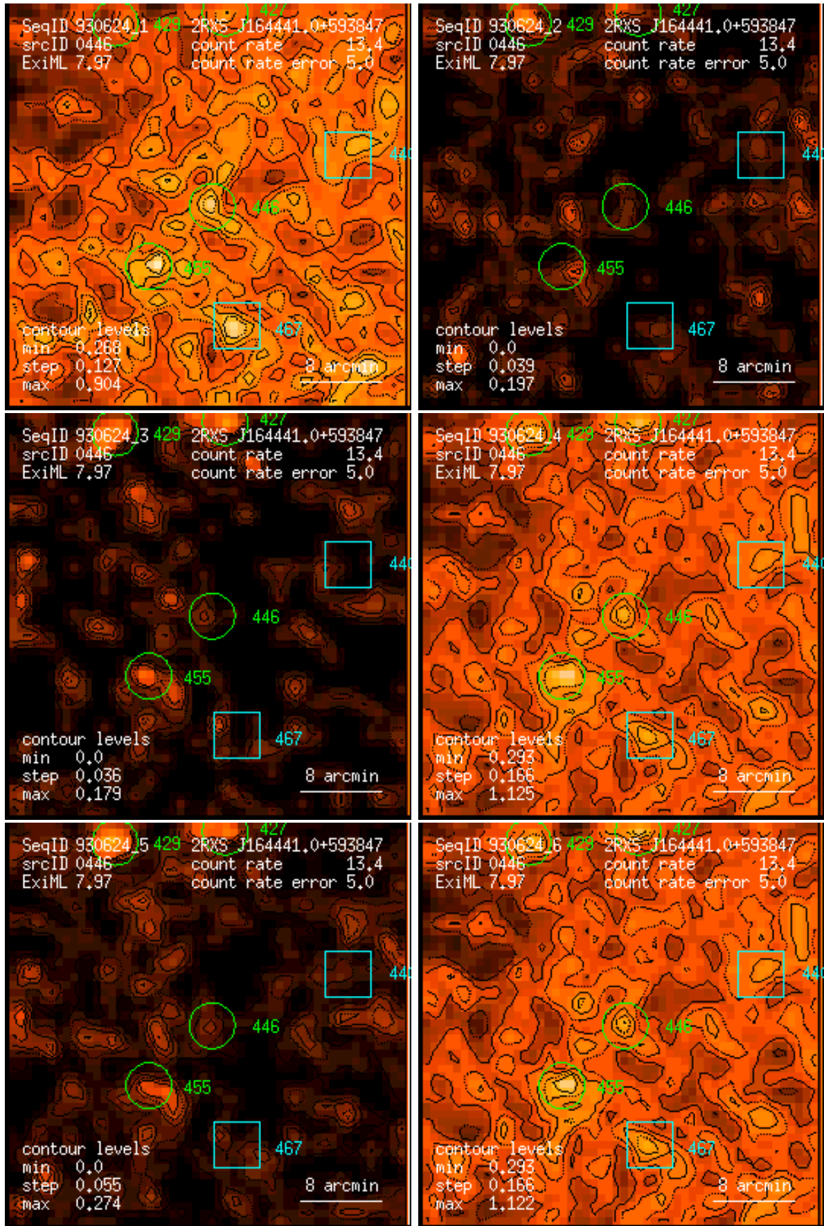
Figure 446: RASS 930624: detection 0446: band rate images, Gaussian filter: (1) PSPC channels 11 – 41, (2) 52 – 90, (3) 91 – 201, (4) 11 – 235, (5) 52 – 201, (6) 11 – 201. Broad band rates in counts/ks. Band rate contour levels in counts/ks/arcmin 2 .
