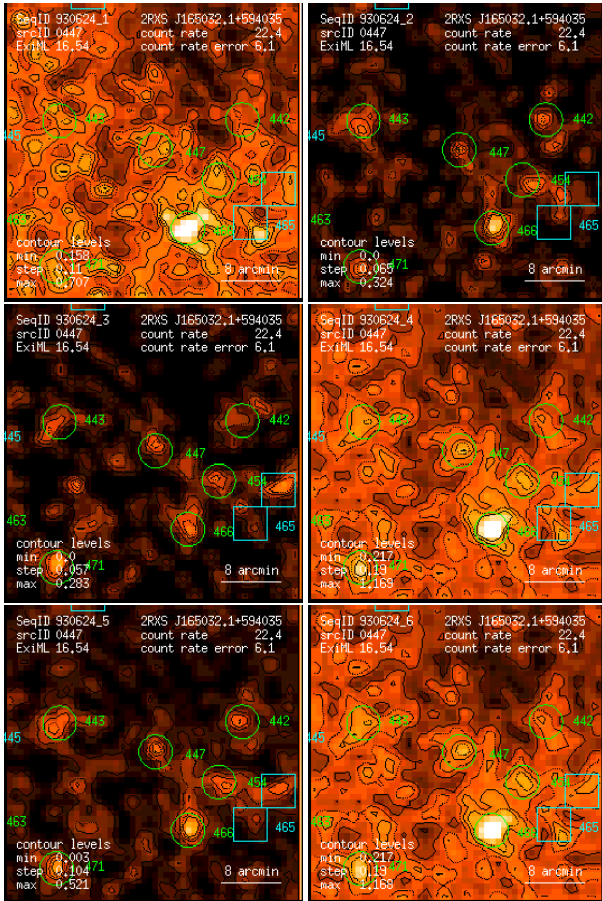
Figure 447: RASS 930624: detection 0447: band rate images, Gaussian filter: (1) PSPC channels 11 – 41, (2) 52 – 90, (3) 91 – 201, (4) 11 – 235, (5) 52 – 201, (6) 11 – 201. Broad band rates in counts/ks. Band rate contour levels in counts/ks/arcmin 2 .
