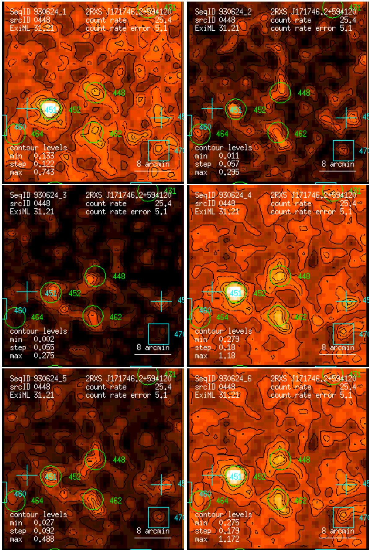
Figure 448: RASS 930624: detection 0448: band rate images, Gaussian filter: (1) PSPC channels 11 – 41, (2) 52 – 90, (3) 91 – 201, (4) 11 – 235, (5) 52 – 201, (6) 11 – 201. Broad band rates in counts/ks. Band rate contour levels in counts/ks/arcmin 2 .
