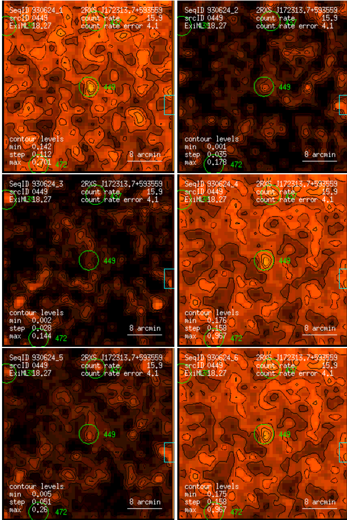
Figure 449: RASS 930624: detection 0449: band rate images, Gaussian filter: (1) PSPC channels 11 – 41, (2) 52 – 90, (3) 91 – 201, (4) 11 – 235, (5) 52 – 201, (6) 11 – 201. Broad band rates in counts/ks. Band rate contour levels in counts/ks/arcmin 2 .
