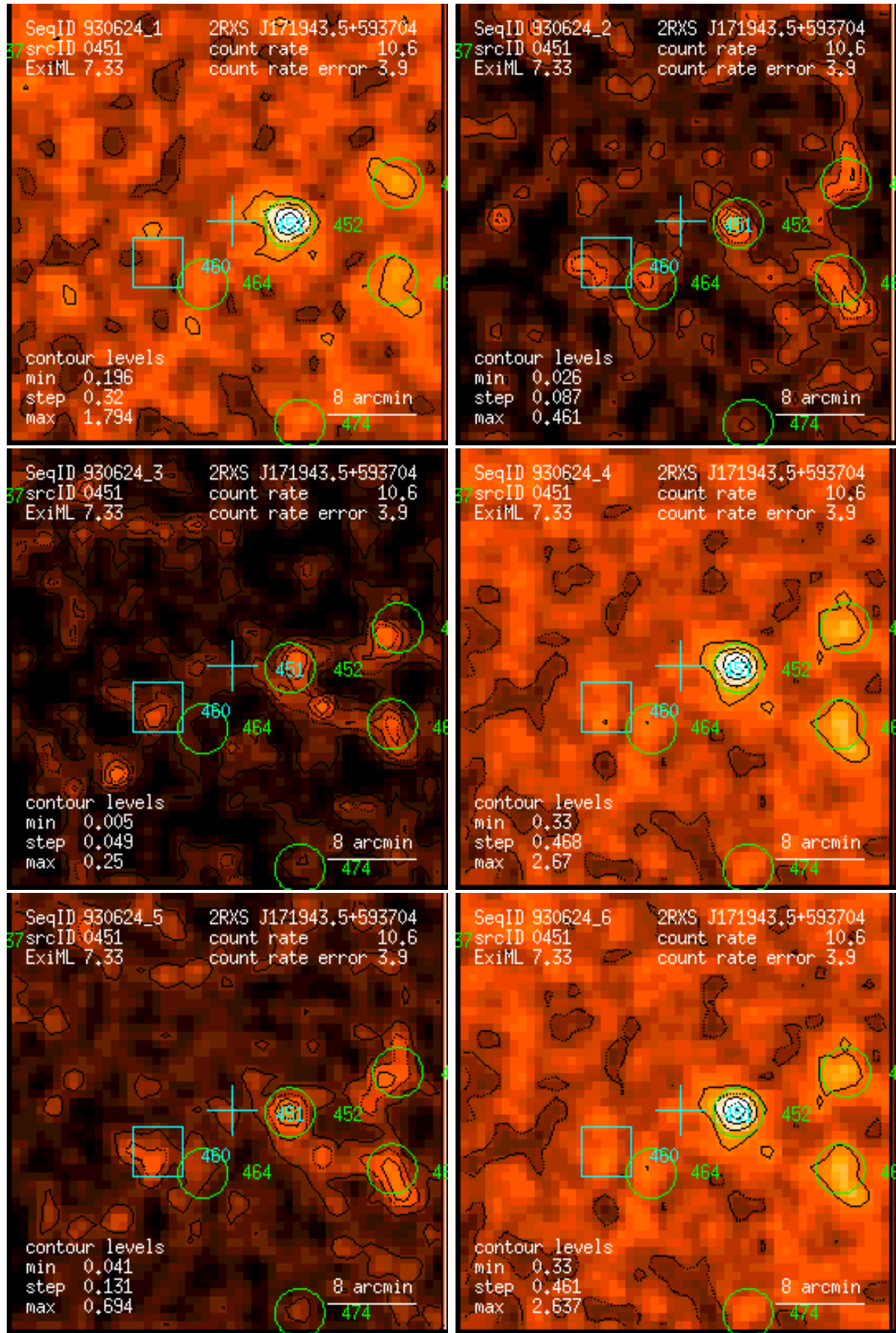
Figure 451: RASS 930624: detection 0451: band rate images, Gaussian filter: (1) PSPC channels 11 – 41, (2) 52 – 90, (3) 91 – 201, (4) 11 – 235, (5) 52 – 201, (6) 11 – 201. Broad band rates in counts/ks. Band rate contour levels in counts/ks/arcmin 2 .
