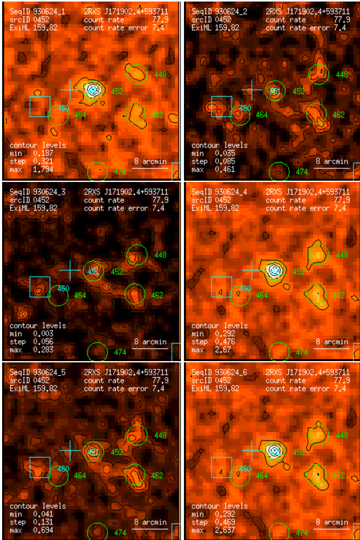
Figure 452: RASS 930624: detection 0452: band rate images, Gaussian filter: (1) PSPC channels 11 – 41, (2) 52 – 90, (3) 91 – 201, (4) 11 – 235, (5) 52 – 201, (6) 11 – 201. Broad band rates in counts/ks. Band rate contour levels in counts/ks/arcmin 2 .
