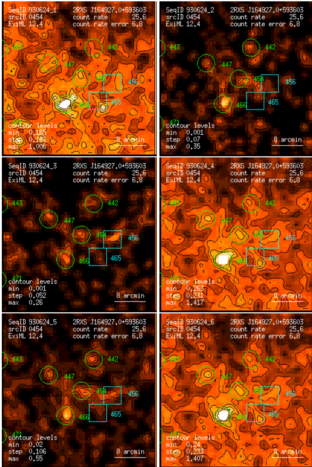
Figure 454: RASS 930624: detection 0454: band rate images, Gaussian filter: (1) PSPC channels 11 – 41, (2) 52 – 90, (3) 91 – 201, (4) 11 – 235, (5) 52 – 201, (6) 11 – 201. Broad band rates in counts/ks. Band rate contour levels in counts/ks/arcmin 2 .
