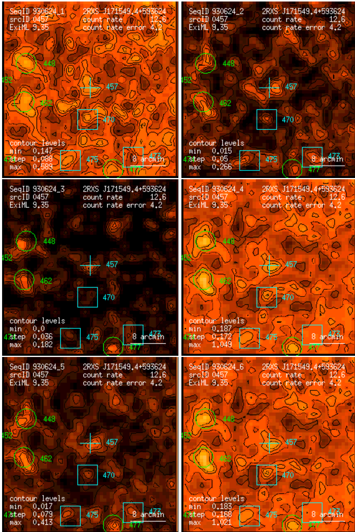
Figure 457: RASS 930624: detection 0457: band rate images, Gaussian filter: (1) PSPC channels 11 – 41, (2) 52 – 90, (3) 91 – 201, (4) 11 – 235, (5) 52 – 201, (6) 11 – 201. Broad band rates in counts/ks. Band rate contour levels in counts/ks/arcmin 2 .
