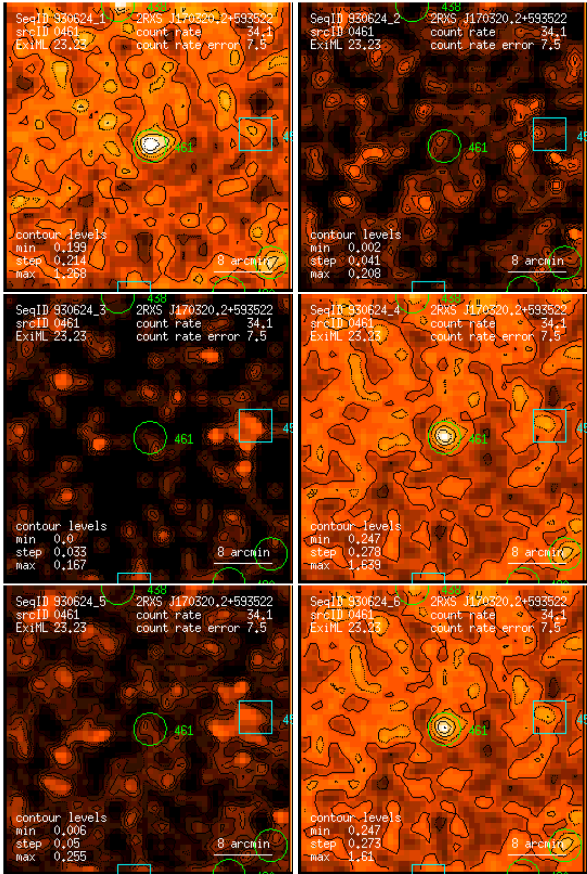
Figure 461: RASS 930624: detection 0461: band rate images, Gaussian filter: (1) PSPC channels 11 – 41, (2) 52 – 90, (3) 91 – 201, (4) 11 – 235, (5) 52 – 201, (6) 11 – 201. Broad band rates in counts/ks. Band rate contour levels in counts/ks/arcmin 2 .
