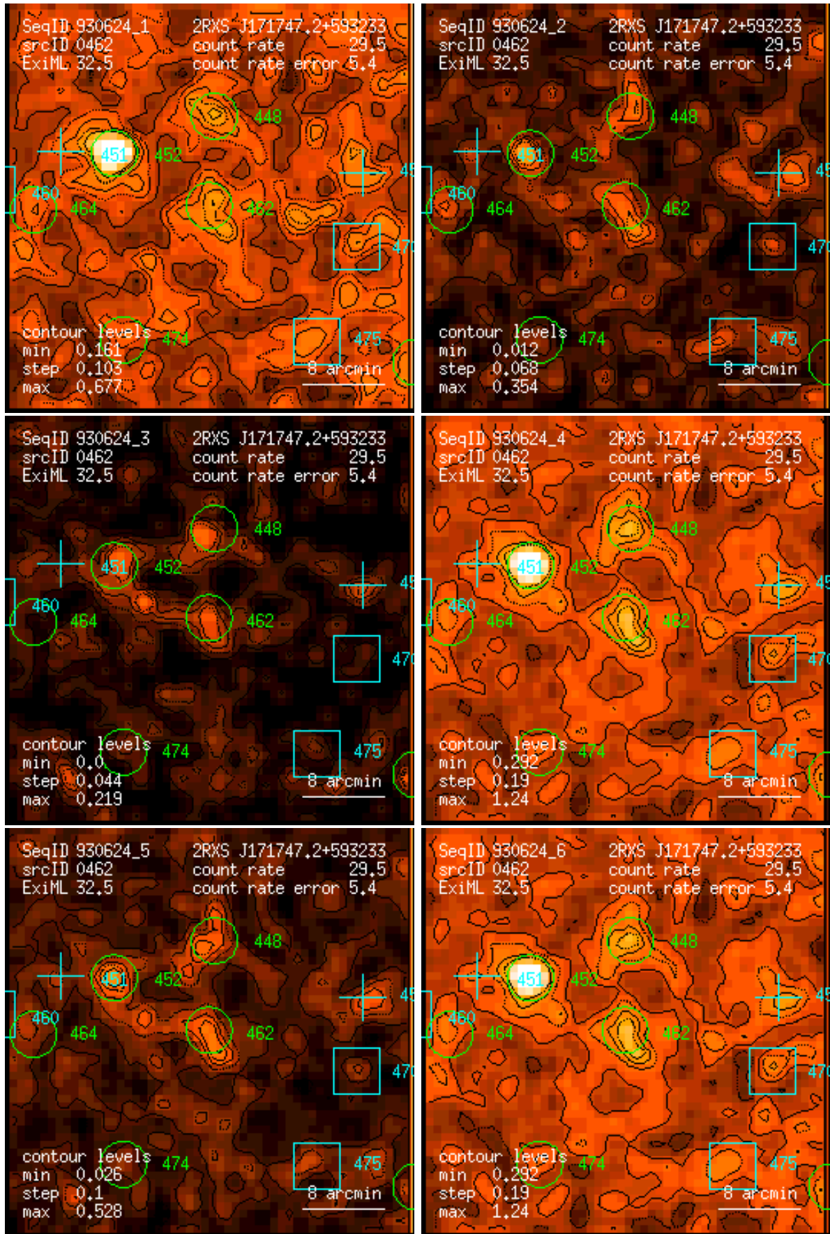
Figure 462: RASS 930624: detection 0462: band rate images, Gaussian filter: (1) PSPC channels 11 – 41, (2) 52 – 90, (3) 91 – 201, (4) 11 – 235, (5) 52 – 201, (6) 11 – 201. Broad band rates in counts/ks. Band rate contour levels in counts/ks/arcmin 2 .
