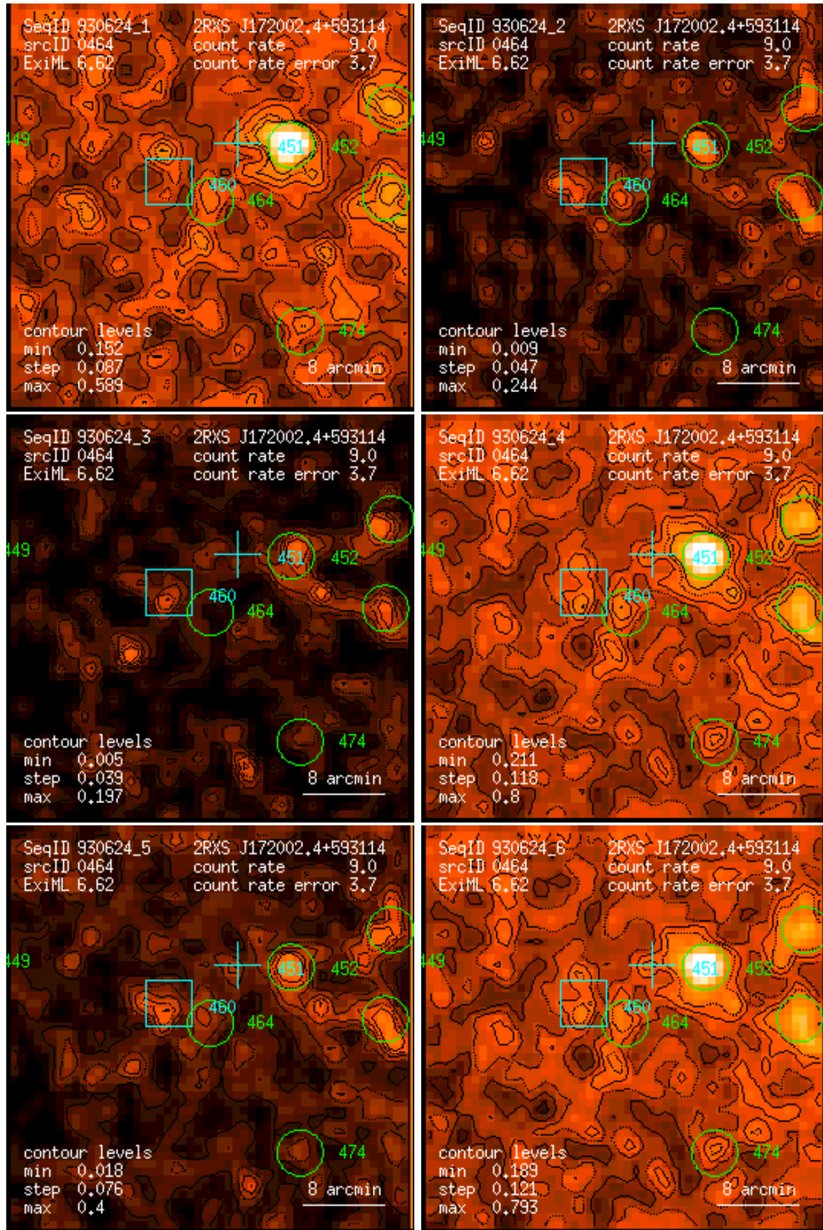
Figure 464: RASS 930624: detection 0464: band rate images, Gaussian filter: (1) PSPC channels 11 – 41, (2) 52 – 90, (3) 91 – 201, (4) 11 – 235, (5) 52 – 201, (6) 11 – 201. Broad band rates in counts/ks. Band rate contour levels in counts/ks/arcmin 2 .
