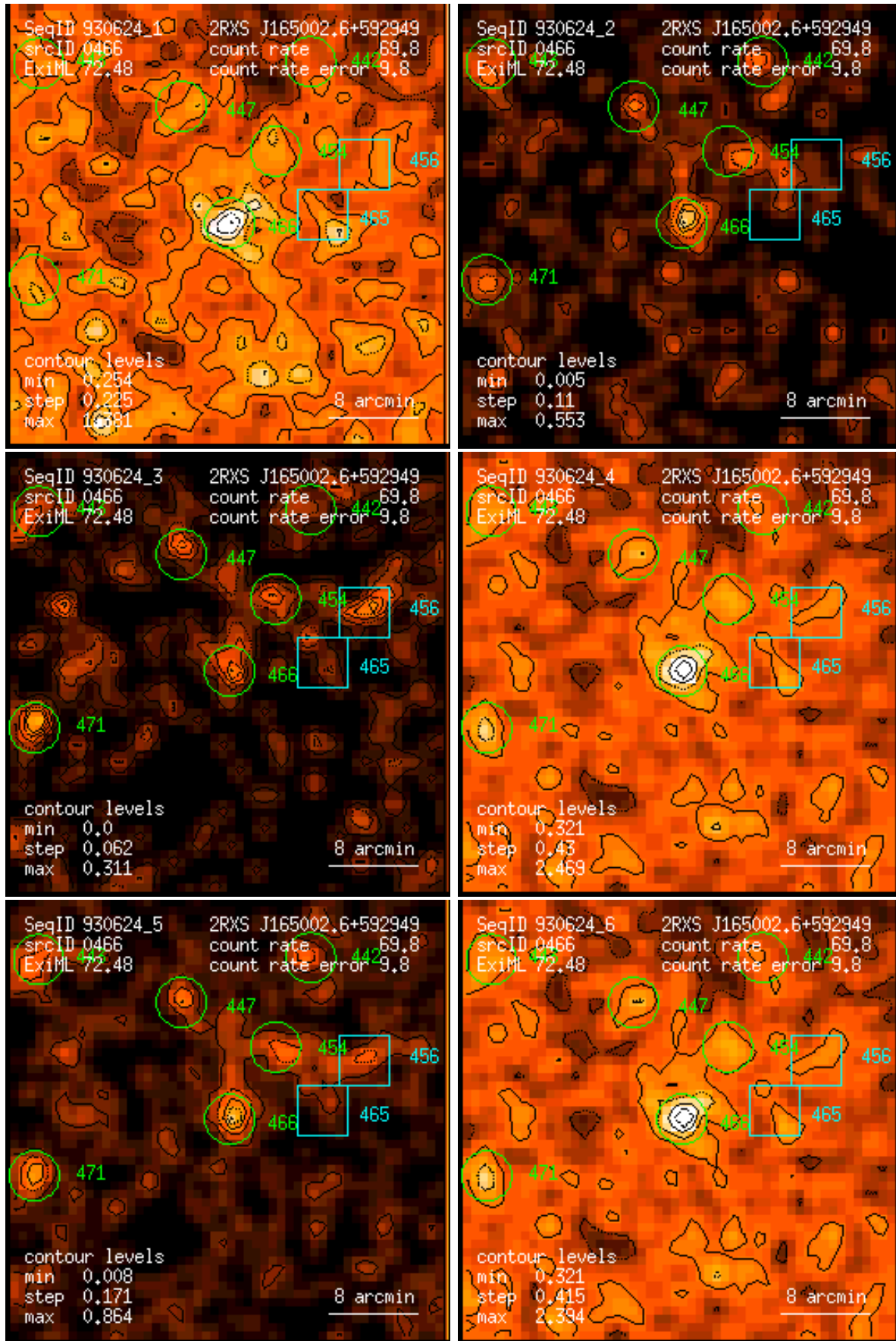
Figure 466: RASS 930624: detection 0466: band rate images, Gaussian filter: (1) PSPC channels 11 – 41, (2) 52 – 90, (3) 91 – 201, (4) 11 – 235, (5) 52 – 201, (6) 11 – 201. Broad band rates in counts/ks. Band rate contour levels in counts/ks/arcmin 2 .
