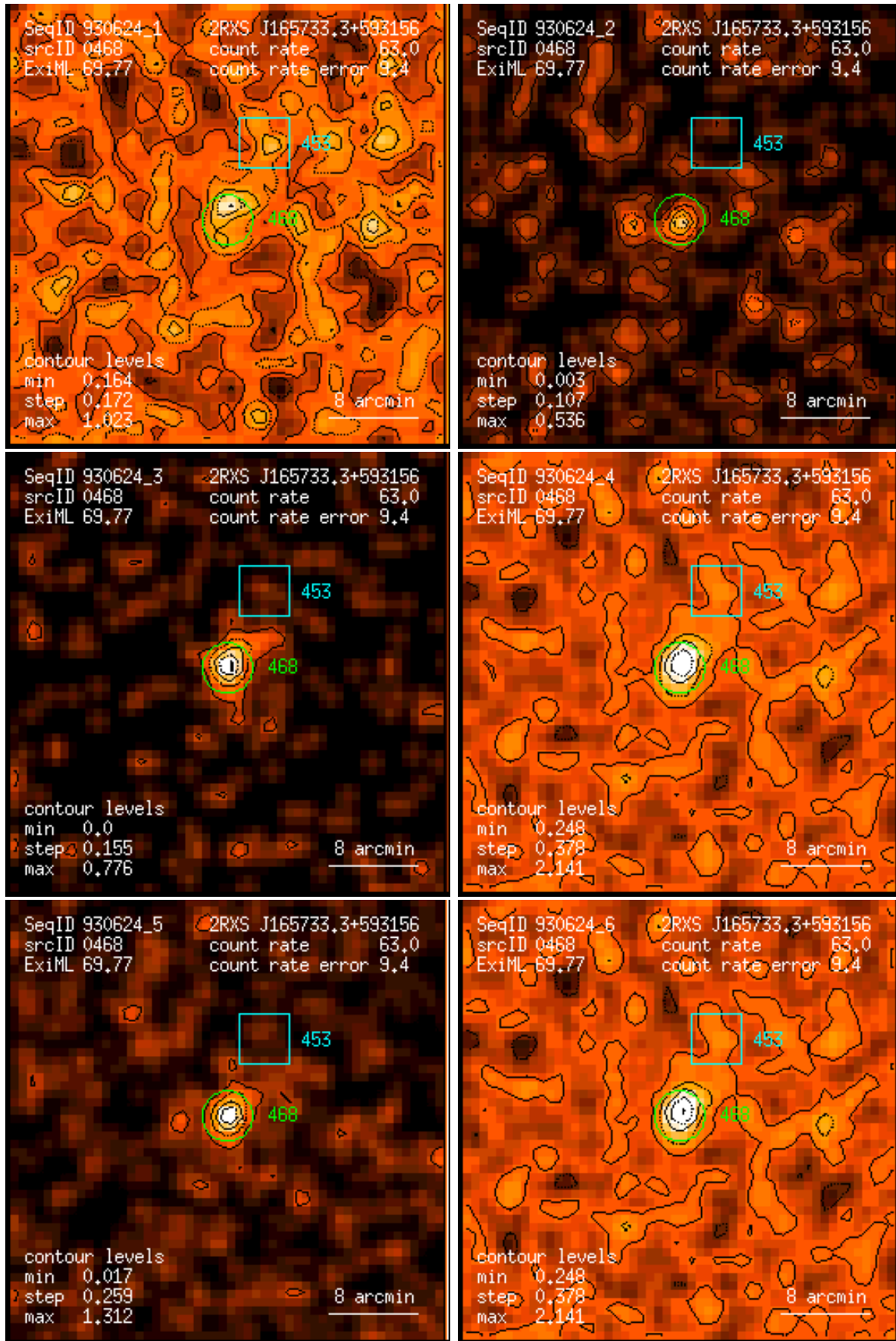
Figure 468: RASS 930624: detection 0468: band rate images, Gaussian filter: (1) PSPC channels 11 – 41, (2) 52 – 90, (3) 91 – 201, (4) 11 – 235, (5) 52 – 201, (6) 11 – 201. Broad band rates in counts/ks. Band rate contour levels in counts/ks/arcmin 2 .
