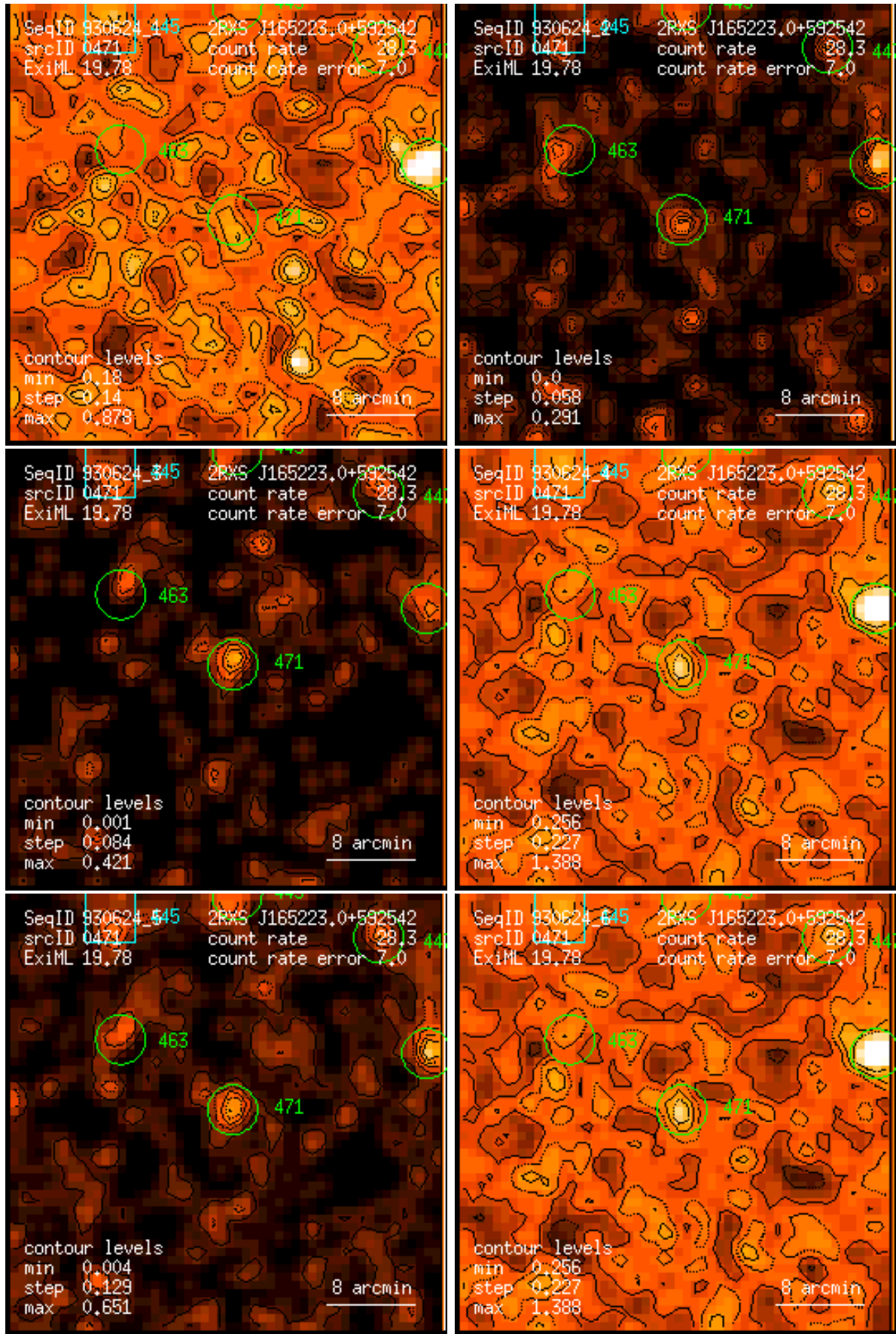
Figure 471: RASS 930624: detection 0471: band rate images, Gaussian filter: (1) PSPC channels 11 – 41, (2) 52 – 90, (3) 91 – 201, (4) 11 – 235, (5) 52 – 201, (6) 11 – 201. Broad band rates in counts/ks. Band rate contour levels in counts/ks/arcmin 2 .
