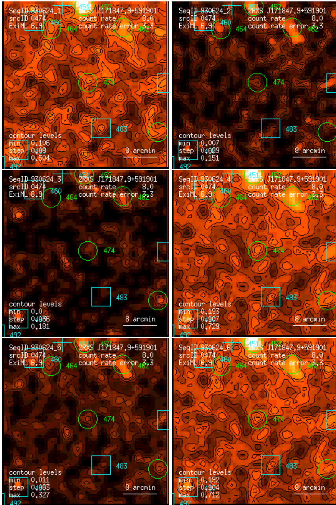
Figure 474: RASS 930624: detection 0474: band rate images, Gaussian filter: (1) PSPC channels 11 – 41, (2) 52 – 90, (3) 91 – 201, (4) 11 – 235, (5) 52 – 201, (6) 11 – 201. Broad band rates in counts/ks. Band rate contour levels in counts/ks/arcmin 2 .
