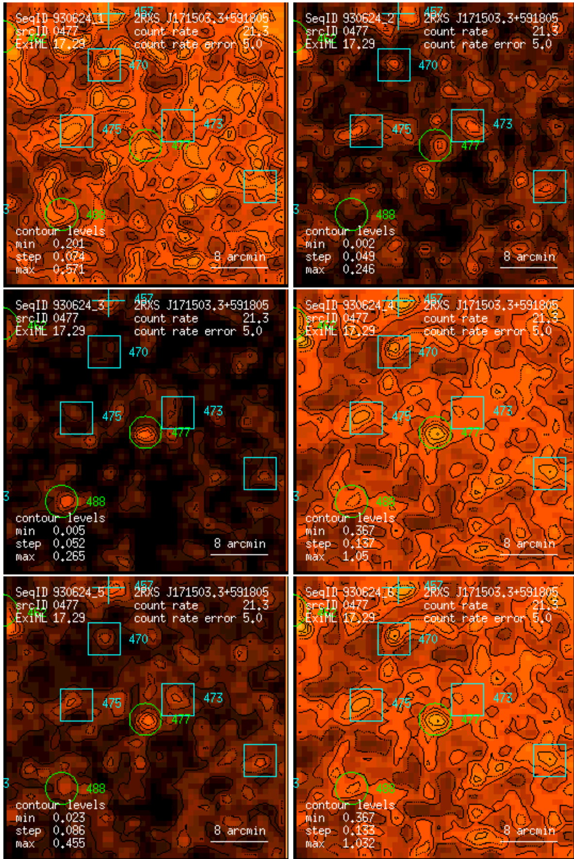
Figure 477: RASS 930624: detection 0477: band rate images, Gaussian filter: (1) PSPC channels 11 – 41, (2) 52 – 90, (3) 91 – 201, (4) 11 – 235, (5) 52 – 201, (6) 11 – 201. Broad band rates in counts/ks. Band rate contour levels in counts/ks/arcmin 2 .
