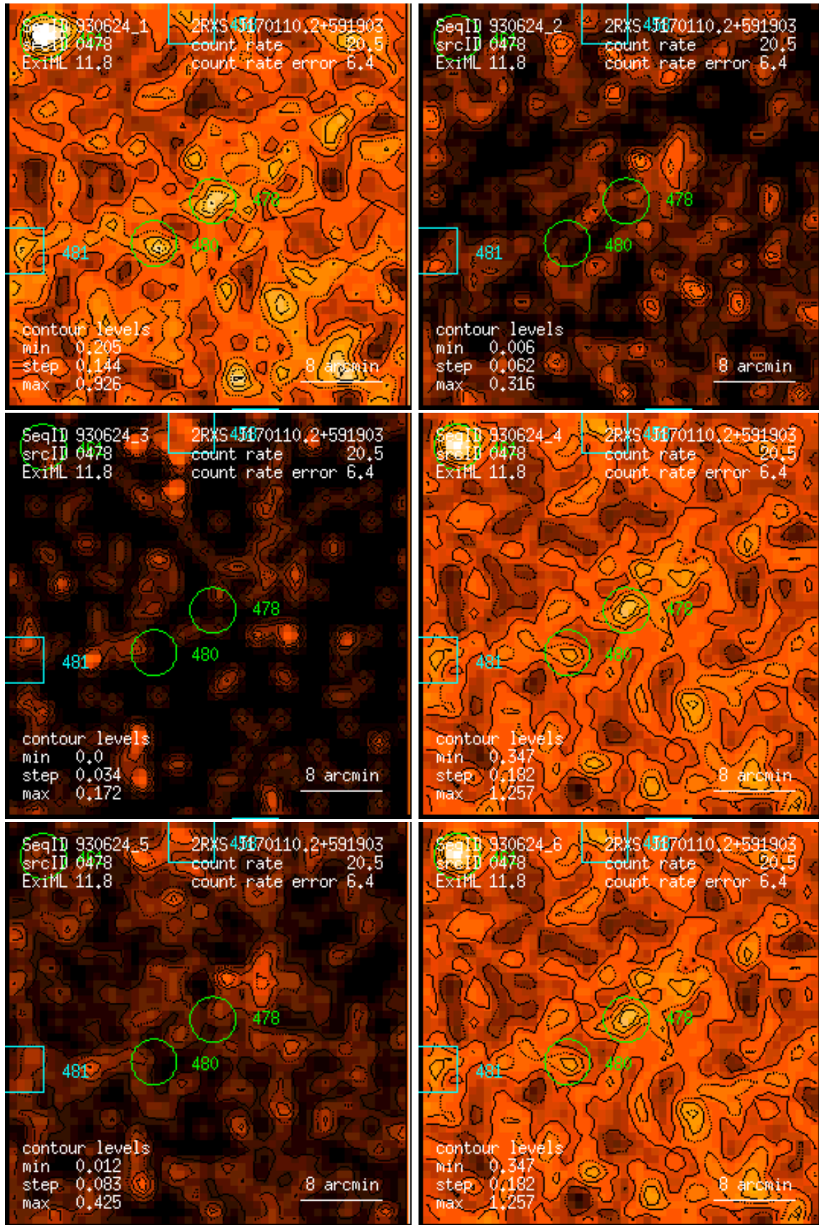
Figure 478: RASS 930624: detection 0478: band rate images, Gaussian filter: (1) PSPC channels 11 – 41, (2) 52 – 90, (3) 91 – 201, (4) 11 – 235, (5) 52 – 201, (6) 11 – 201. Broad band rates in counts/ks. Band rate contour levels in counts/ks/arcmin 2 .
