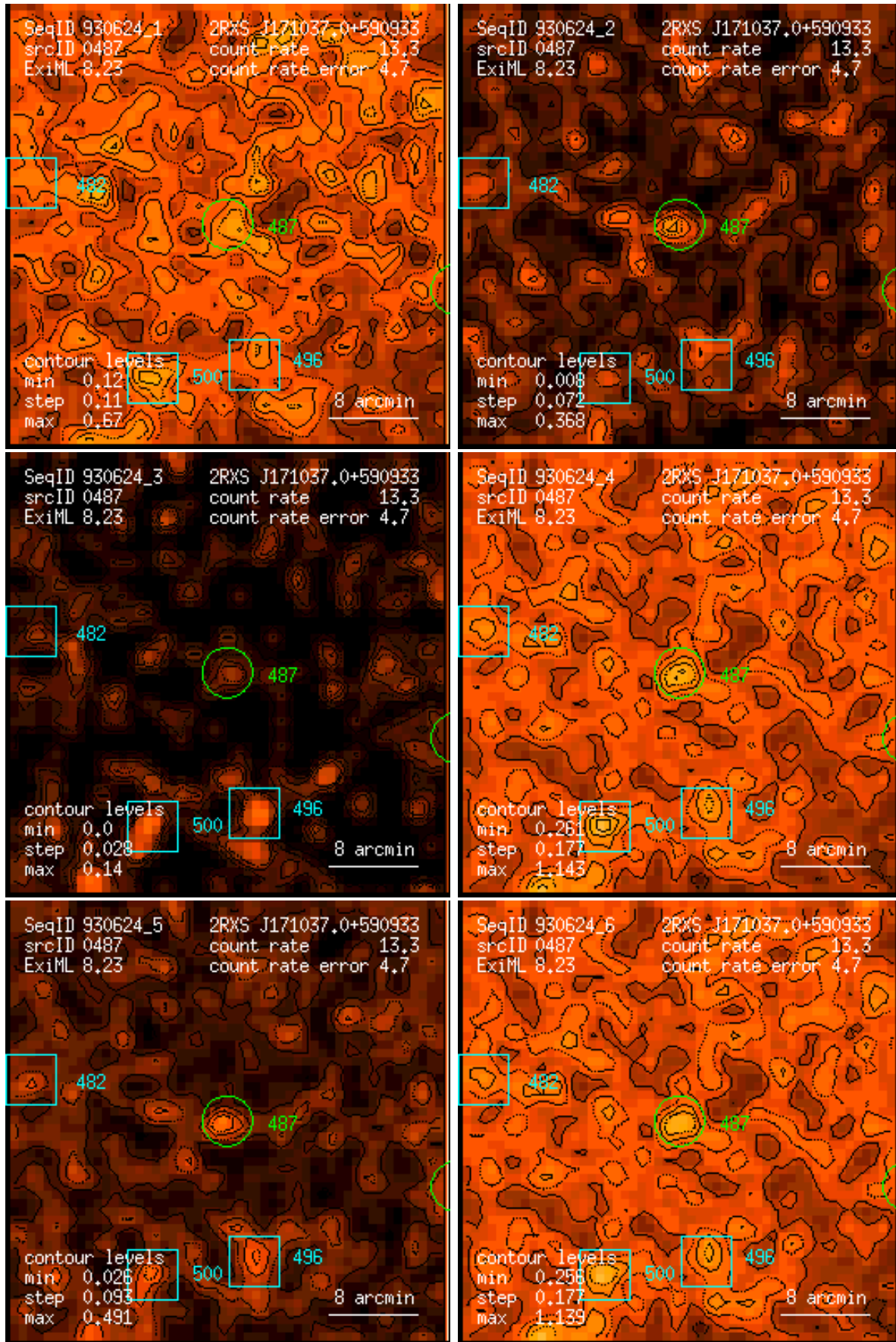
Figure 487: RASS 930624: detection 0487: band rate images, Gaussian filter: (1) PSPC channels 11 – 41, (2) 52 – 90, (3) 91 – 201, (4) 11 – 235, (5) 52 – 201, (6) 11 – 201. Broad band rates in counts/ks. Band rate contour levels in counts/ks/arcmin 2 .
