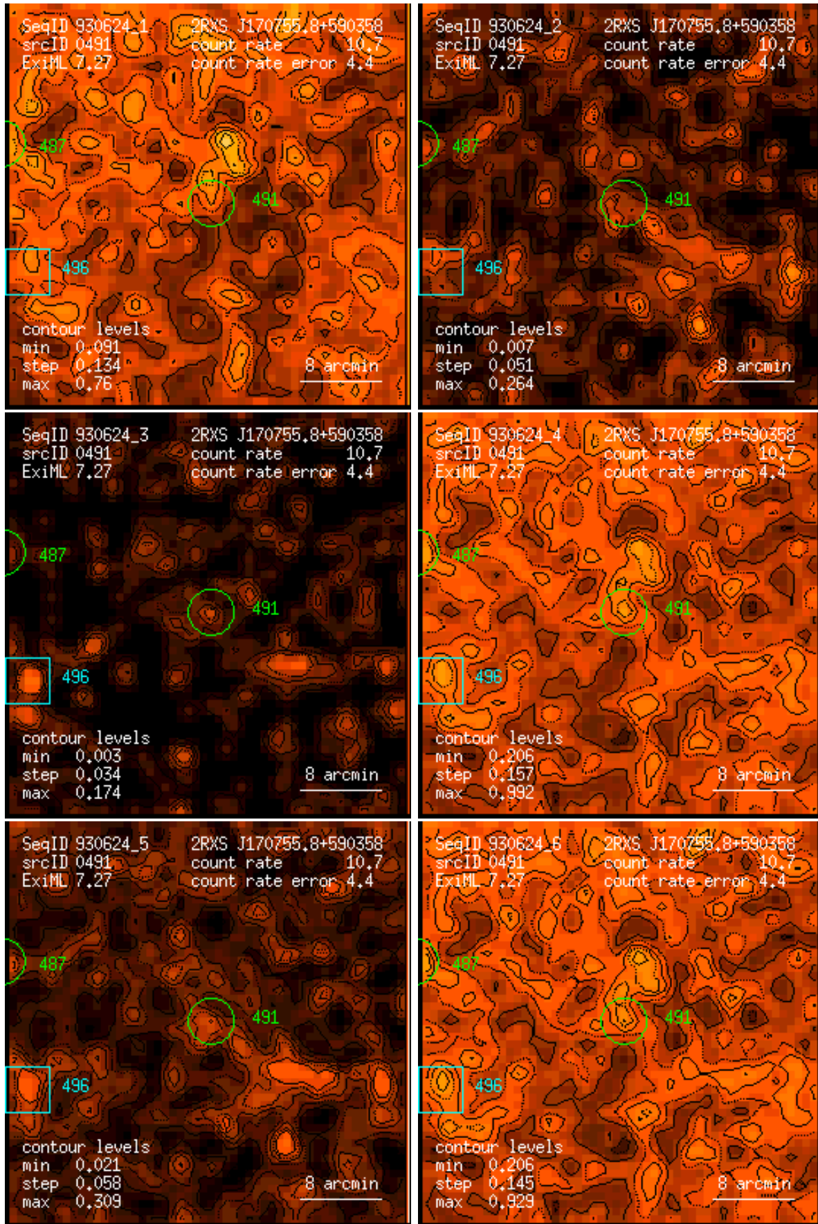
Figure 491: RASS 930624: detection 0491: band rate images, Gaussian filter: (1) PSPC channels 11 – 41, (2) 52 – 90, (3) 91 – 201, (4) 11 – 235, (5) 52 – 201, (6) 11 – 201. Broad band rates in counts/ks. Band rate contour levels in counts/ks/arcmin 2 .
