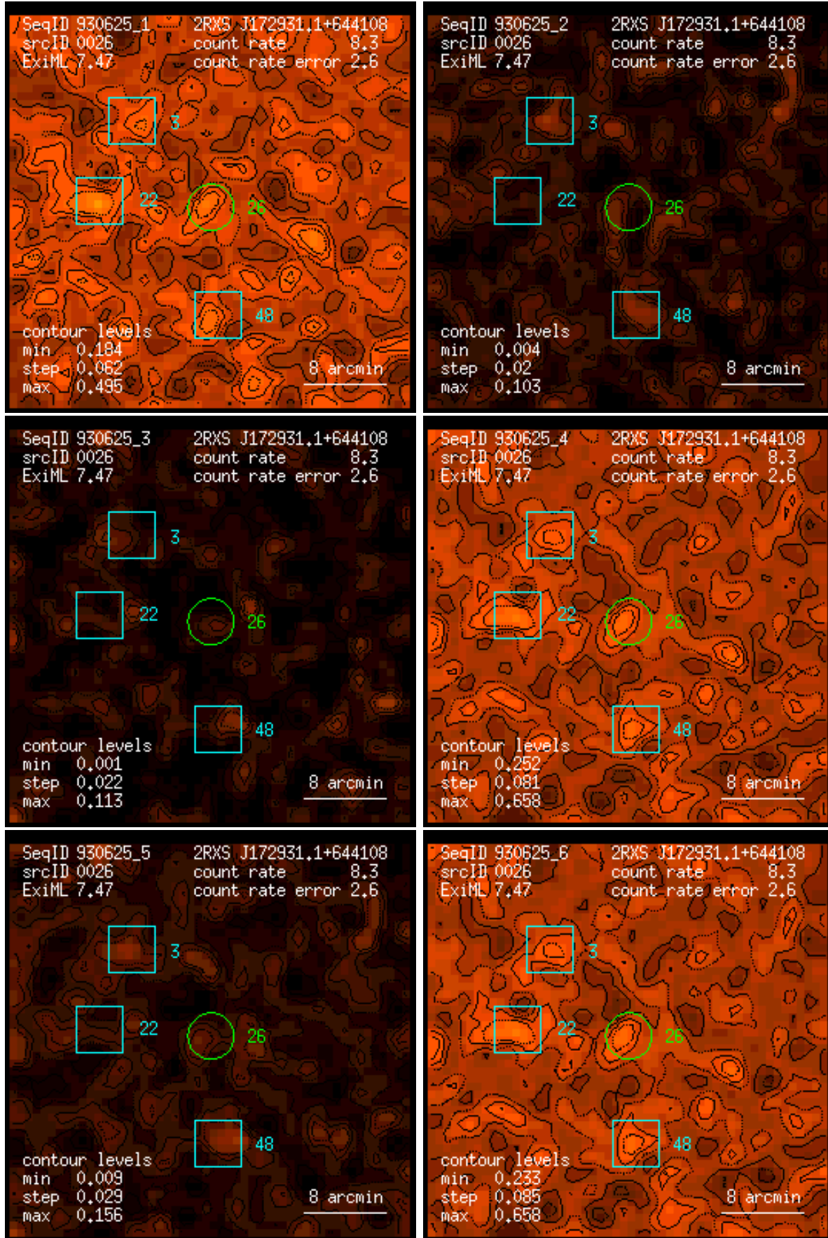
Figure 26: RASS 930625: detection 0026: band rate images, Gaussian filter: (1) PSPC channels 11 – 41, (2) 52 – 90, (3) 91 – 201, (4) 11 – 235, (5) 52 – 201, (6) 11 – 201. Broad band rates in counts/ks. Band rate contour levels in counts/ks/arcmin 2 .
