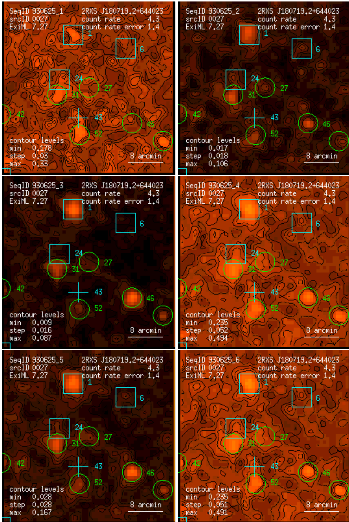
Figure 27: RASS 930625: detection 0027: band rate images, Gaussian filter: (1) PSPC channels 11 – 41, (2) 52 – 90, (3) 91 – 201, (4) 11 – 235, (5) 52 – 201, (6) 11 – 201. Broad band rates in counts/ks. Band rate contour levels in counts/ks/arcmin 2 .
