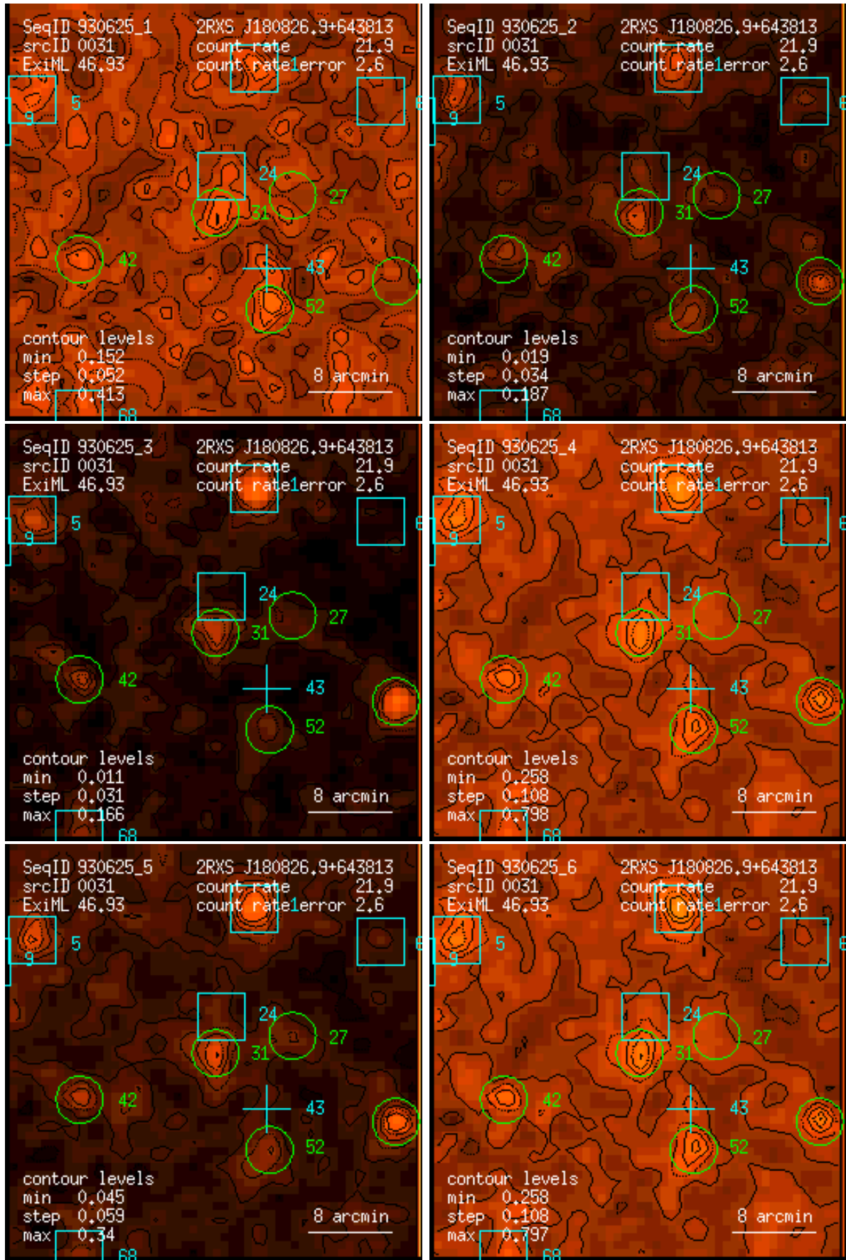
Figure 31: RASS 930625: detection 0031: band rate images, Gaussian filter: (1) PSPC channels 11 – 41, (2) 52 – 90, (3) 91 – 201, (4) 11 – 235, (5) 52 – 201, (6) 11 – 201. Broad band rates in counts/ks. Band rate contour levels in counts/ks/arcmin 2 .
